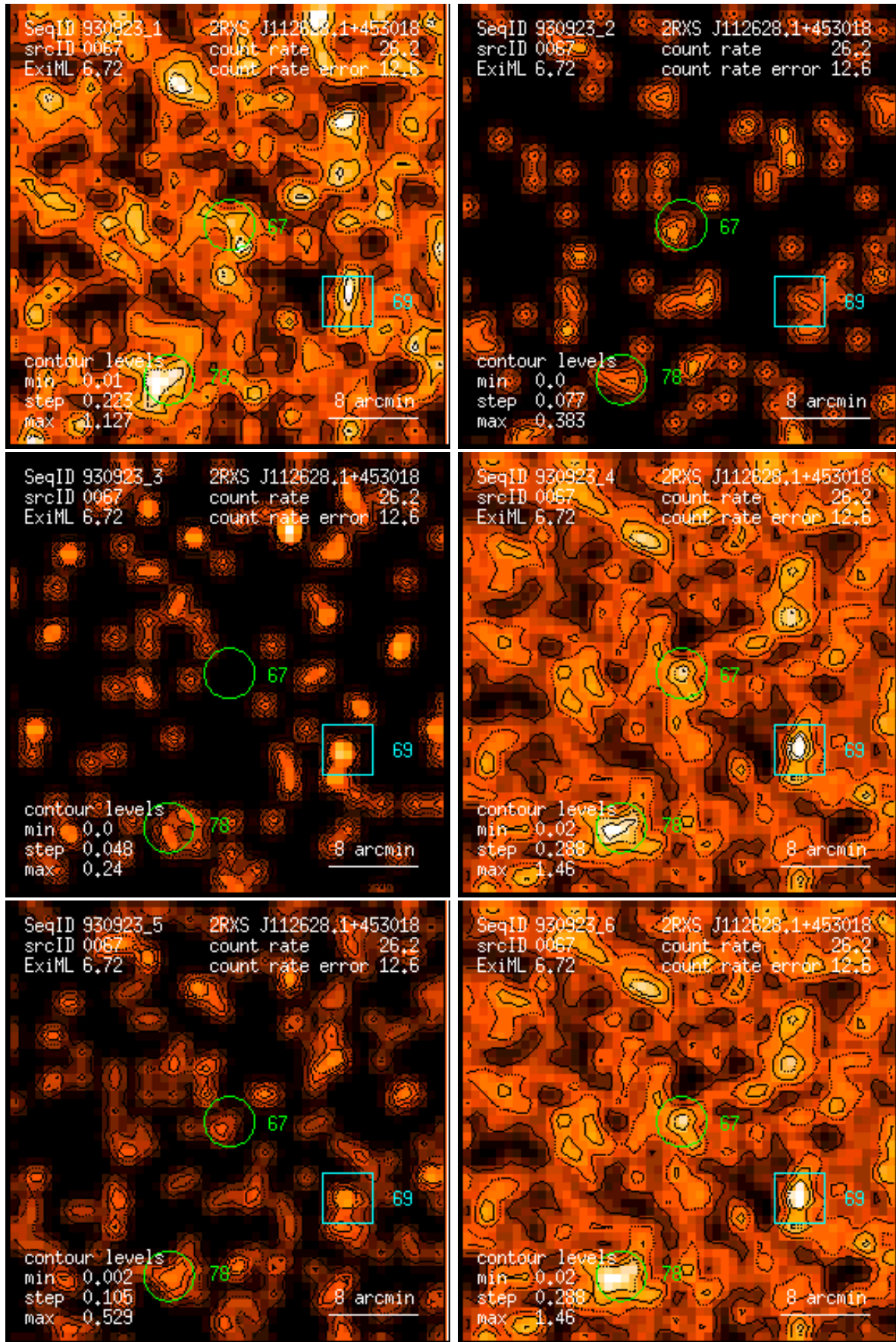
Figure 67: RASS 930923: detection 0067: band rate images, Gaussian filter: (1) PSPC channels 11 – 41, (2) 52 – 90, (3) 91 – 201, (4) 11 – 235, (5) 52 – 201, (6) 11 – 201. Broad band rates in counts/ks. Band rate contour levels in counts/ks/arcmin 2 .
