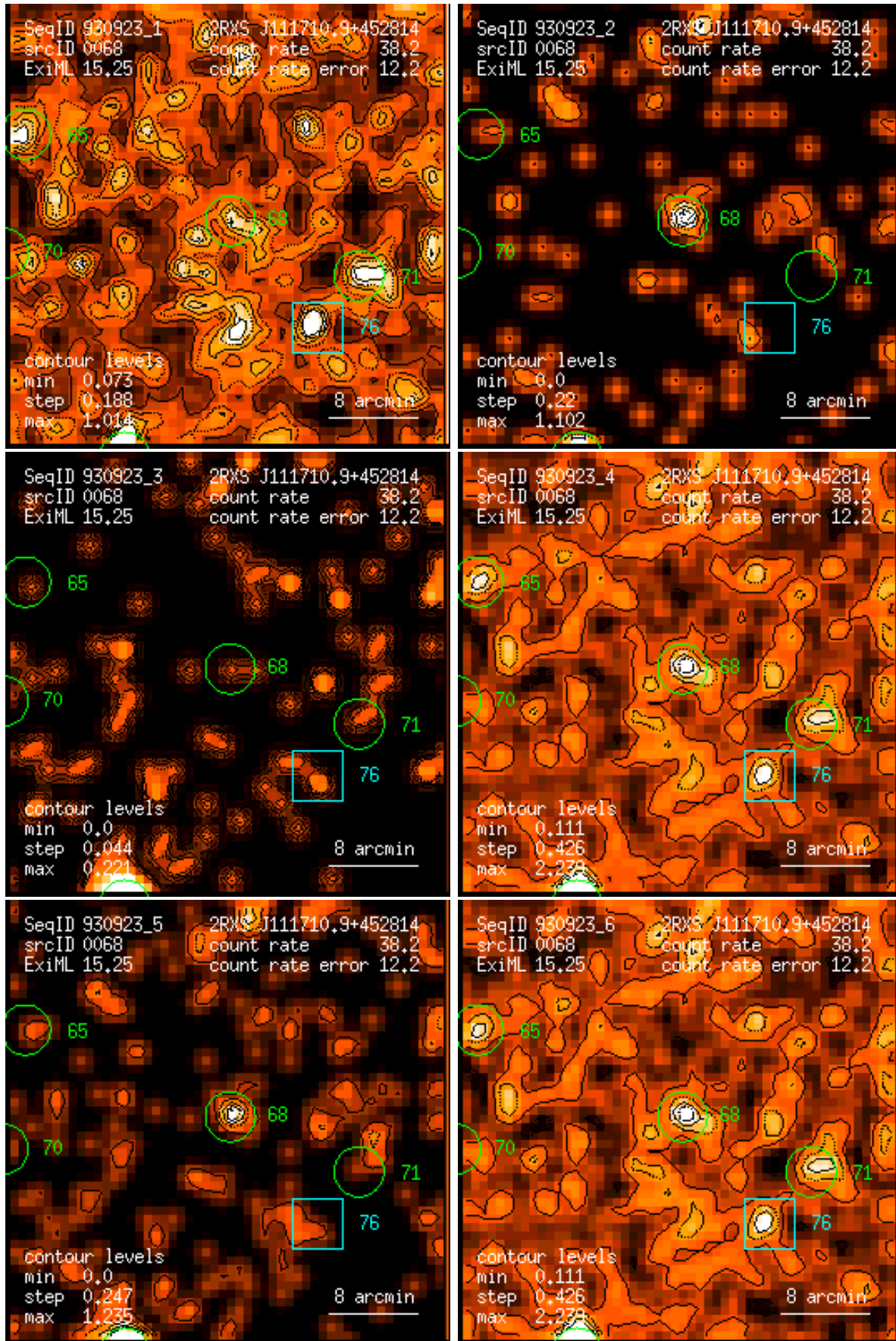
Figure 68: RASS 930923: detection 0068: band rate images, Gaussian filter: (1) PSPC channels 11 – 41, (2) 52 – 90, (3) 91 – 201, (4) 11 – 235, (5) 52 – 201, (6) 11 – 201. Broad band rates in counts/ks. Band rate contour levels in counts/ks/arcmin 2 .
