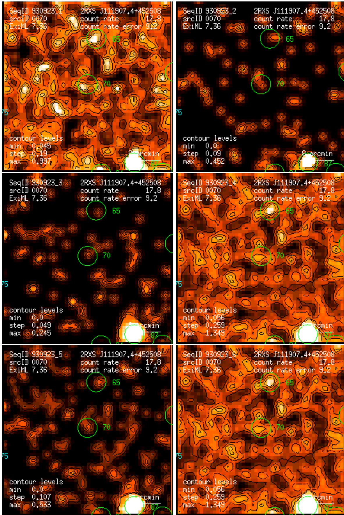
Figure 70: RASS 930923: detection 0070: band rate images, Gaussian filter: (1) PSPC channels 11 – 41, (2) 52 – 90, (3) 91 – 201, (4) 11 – 235, (5) 52 – 201, (6) 11 – 201. Broad band rates in counts/ks. Band rate contour levels in counts/ks/arcmin 2 .
