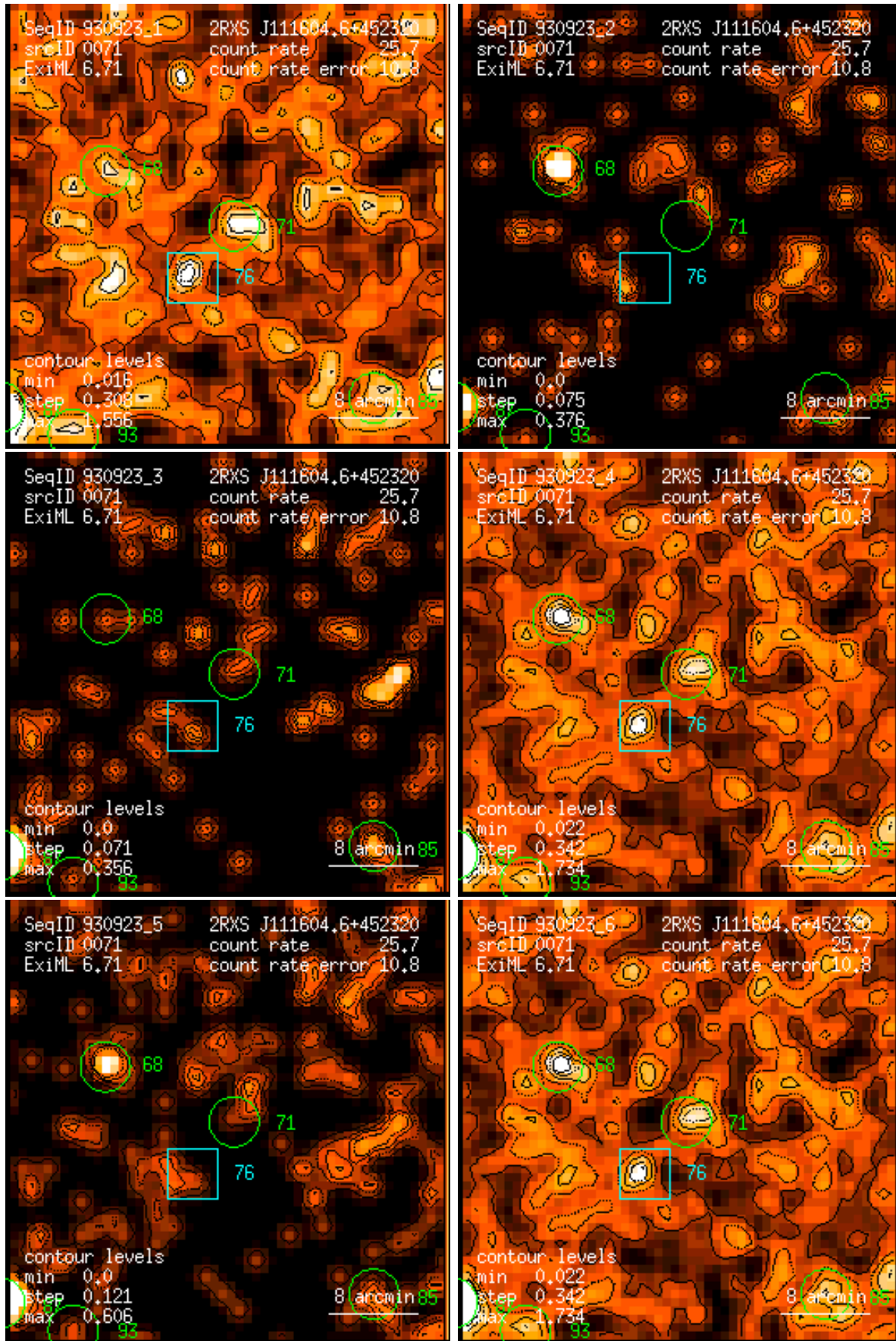
Figure 71: RASS 930923: detection 0071: band rate images, Gaussian filter: (1) PSPC channels 11 – 41, (2) 52 – 90, (3) 91 – 201, (4) 11 – 235, (5) 52 – 201, (6) 11 – 201. Broad band rates in counts/ks. Band rate contour levels in counts/ks/arcmin 2 .
