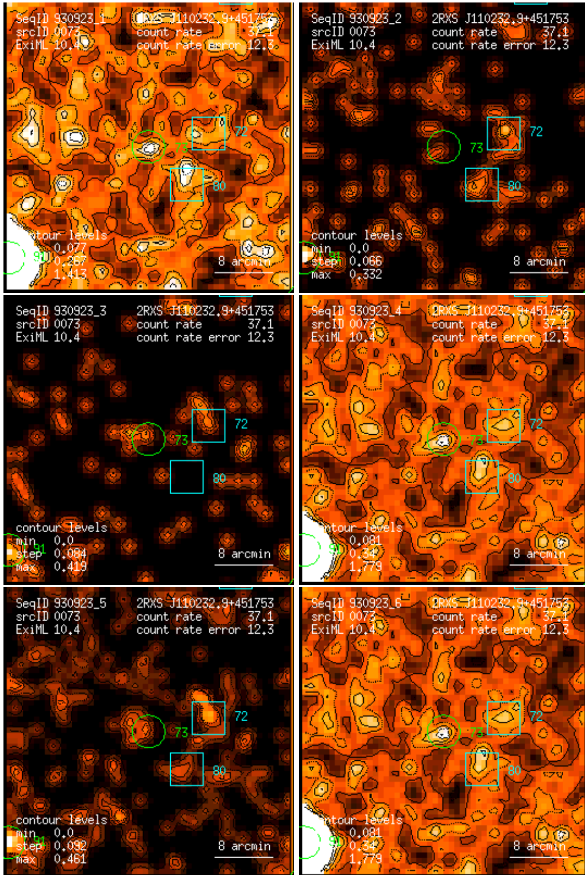
Figure 73: RASS 930923: detection 0073: band rate images, Gaussian filter: (1) PSPC channels 11 – 41, (2) 52 – 90, (3) 91 – 201, (4) 11 – 235, (5) 52 – 201, (6) 11 – 201. Broad band rates in counts/ks. Band rate contour levels in counts/ks/arcmin 2 .
