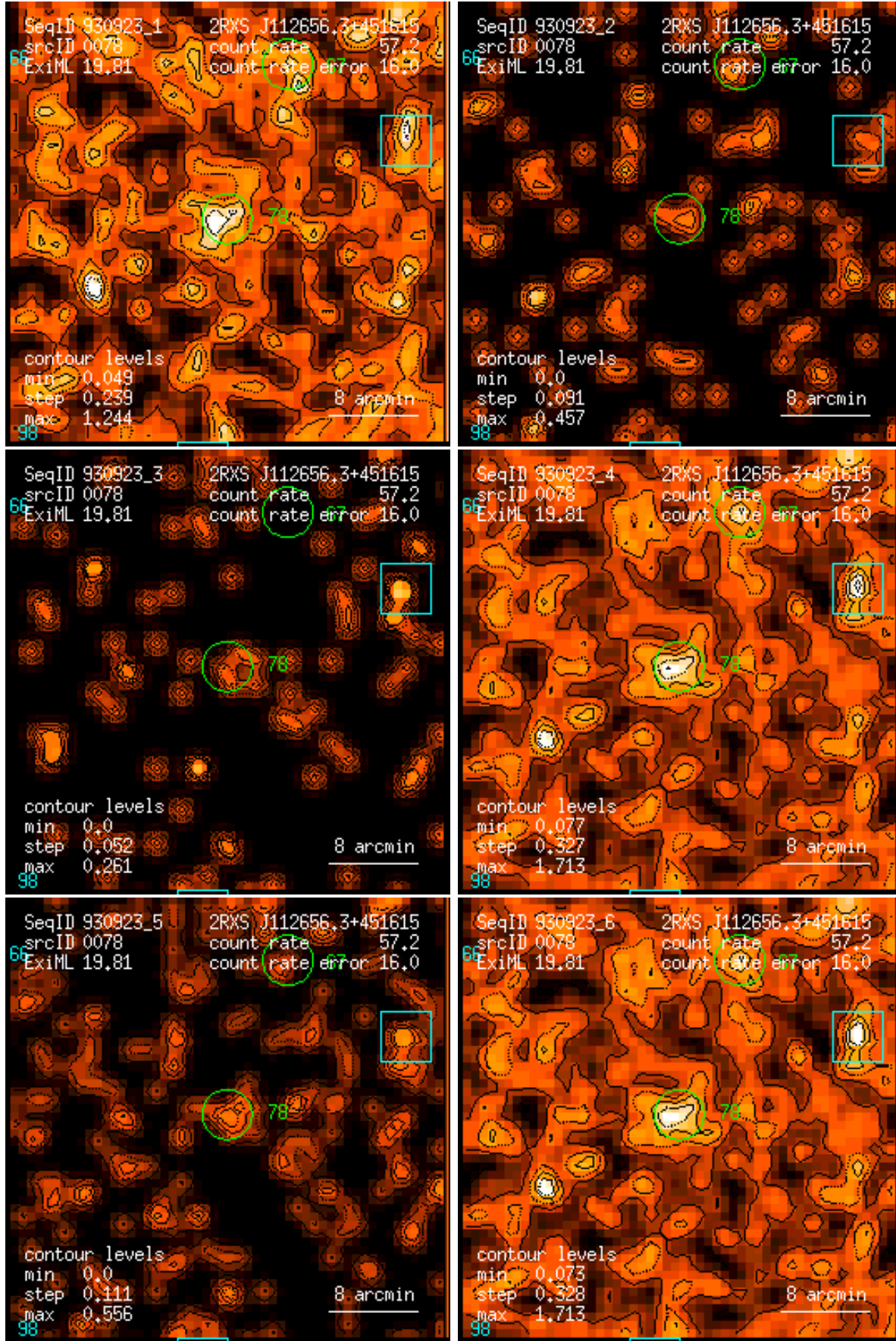
Figure 78: RASS 930923: detection 0078: band rate images, Gaussian filter: (1) PSPC channels 11 – 41, (2) 52 – 90, (3) 91 – 201, (4) 11 – 235, (5) 52 – 201, (6) 11 – 201. Broad band rates in counts/ks. Band rate contour levels in counts/ks/arcmin 2 .
