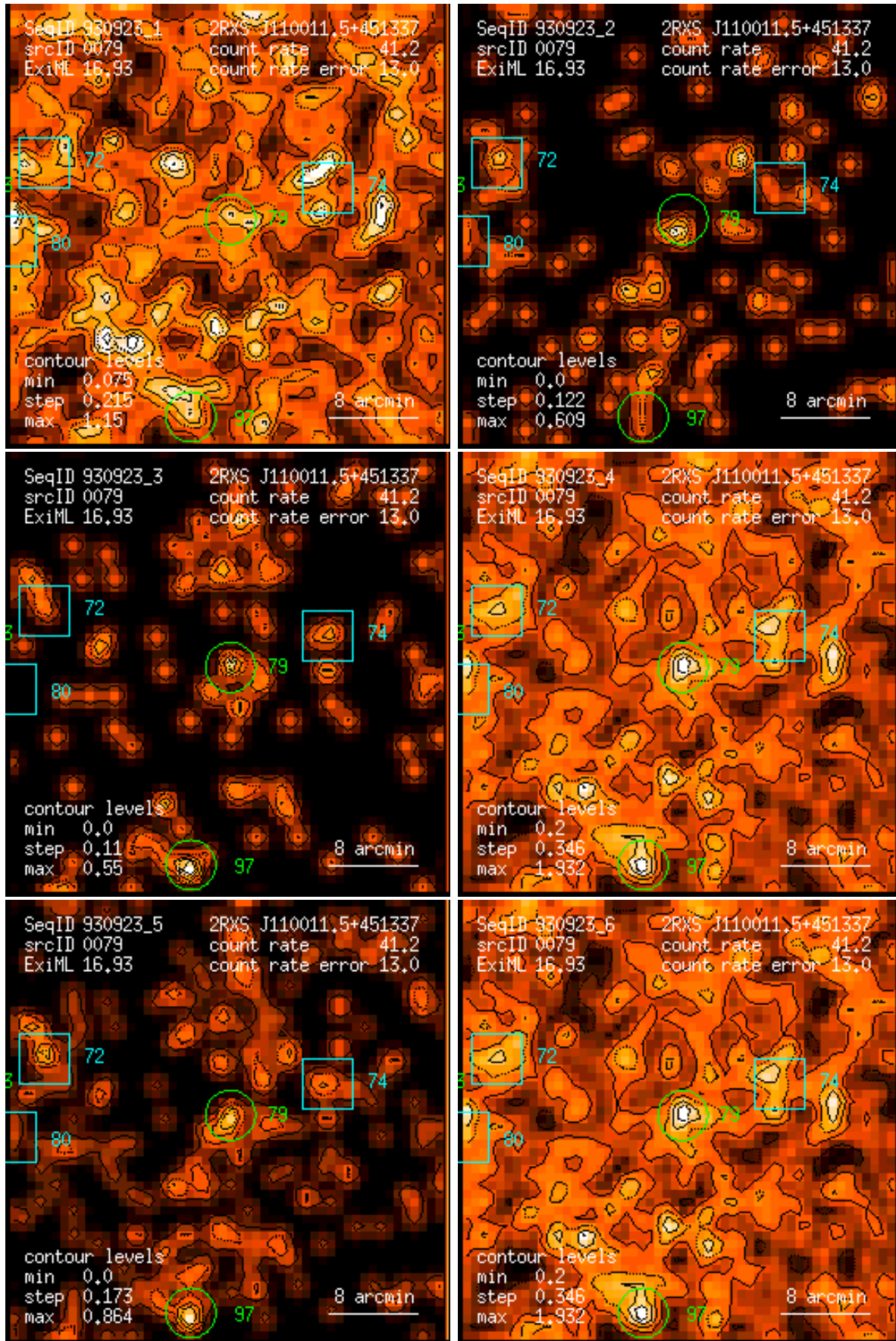
Figure 79: RASS 930923: detection 0079: band rate images, Gaussian filter: (1) PSPC channels 11 – 41, (2) 52 – 90, (3) 91 – 201, (4) 11 – 235, (5) 52 – 201, (6) 11 – 201. Broad band rates in counts/ks. Band rate contour levels in counts/ks/arcmin 2 .
