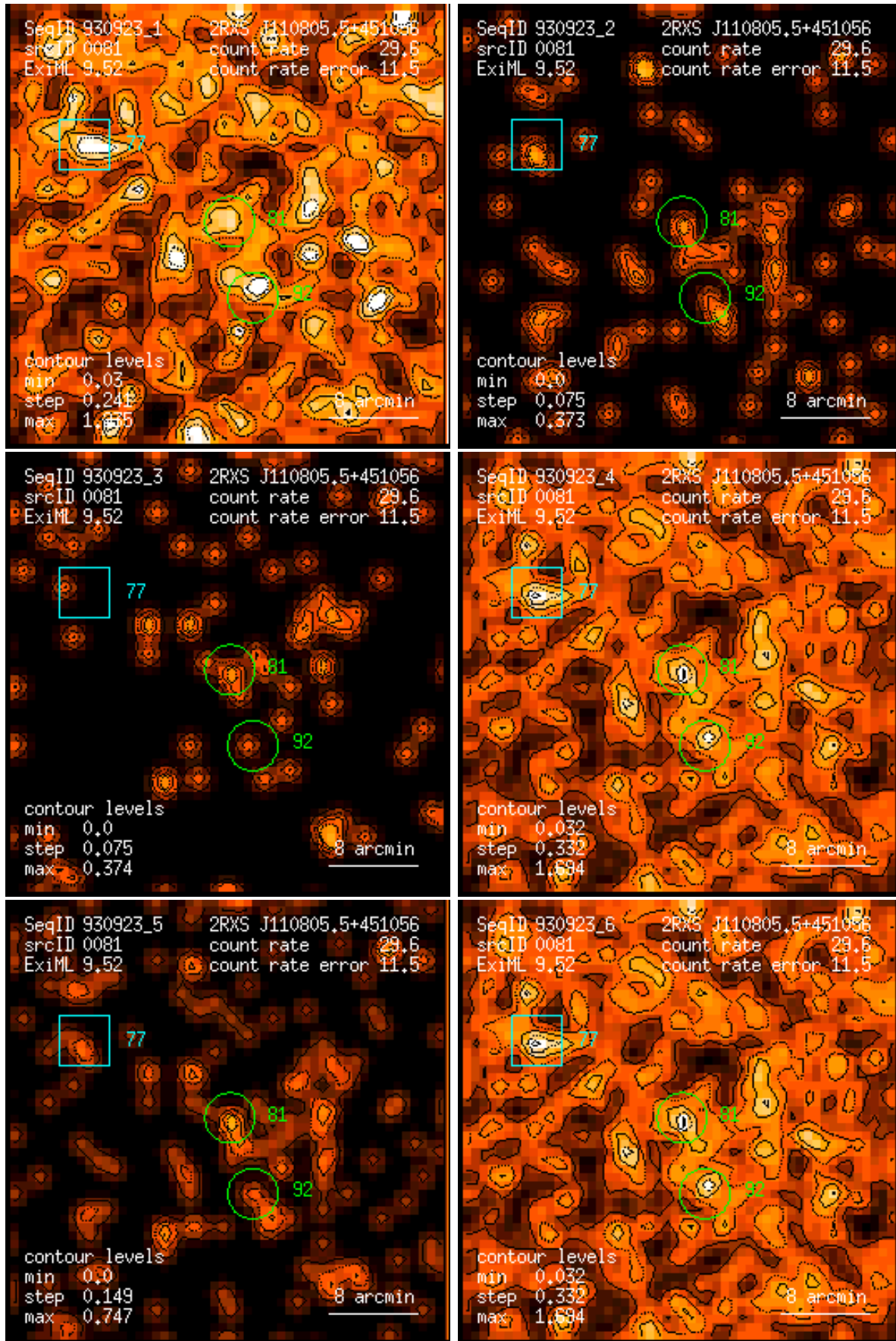
Figure 81: RASS 930923: detection 0081: band rate images, Gaussian filter: (1) PSPC channels 11 – 41, (2) 52 – 90, (3) 91 – 201, (4) 11 – 235, (5) 52 – 201, (6) 11 – 201. Broad band rates in counts/ks. Band rate contour levels in counts/ks/arcmin 2 .
