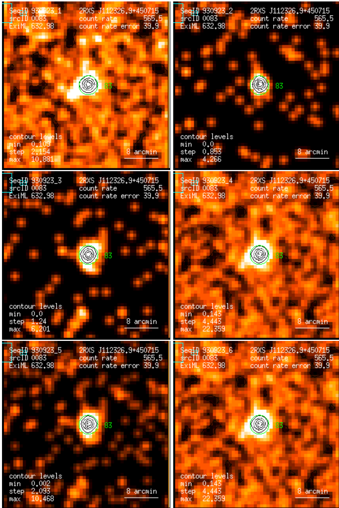
Figure 83: RASS 930923: detection 0083: band rate images, Gaussian filter: (1) PSPC channels 11 – 41, (2) 52 – 90, (3) 91 – 201, (4) 11 – 235, (5) 52 – 201, (6) 11 – 201. Broad band rates in counts/ks. Band rate contour levels in counts/ks/arcmin 2 .
