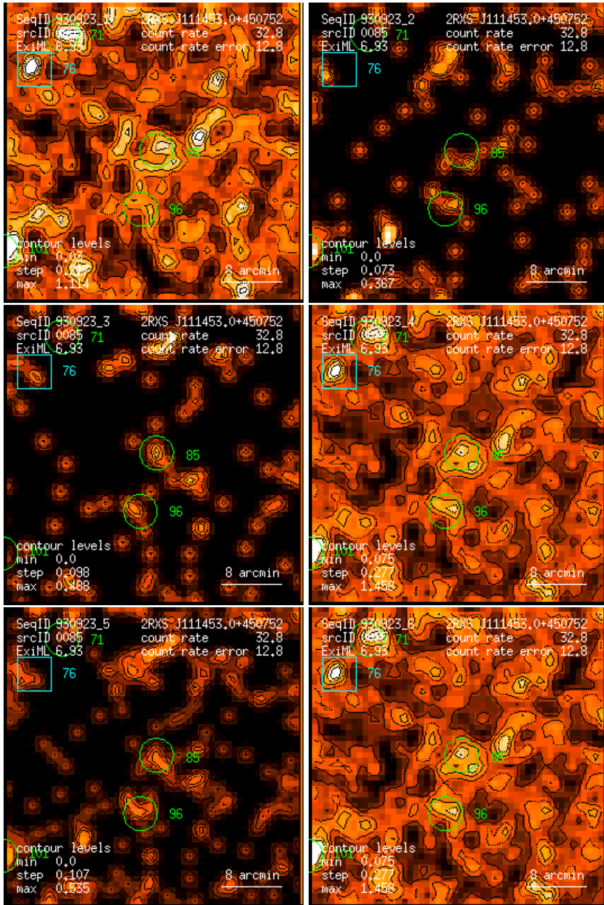
Figure 85: RASS 930923: detection 0085: band rate images, Gaussian filter: (1) PSPC channels 11 – 41, (2) 52 – 90, (3) 91 – 201, (4) 11 – 235, (5) 52 – 201, (6) 11 – 201. Broad band rates in counts/ks. Band rate contour levels in counts/ks/arcmin 2 .
