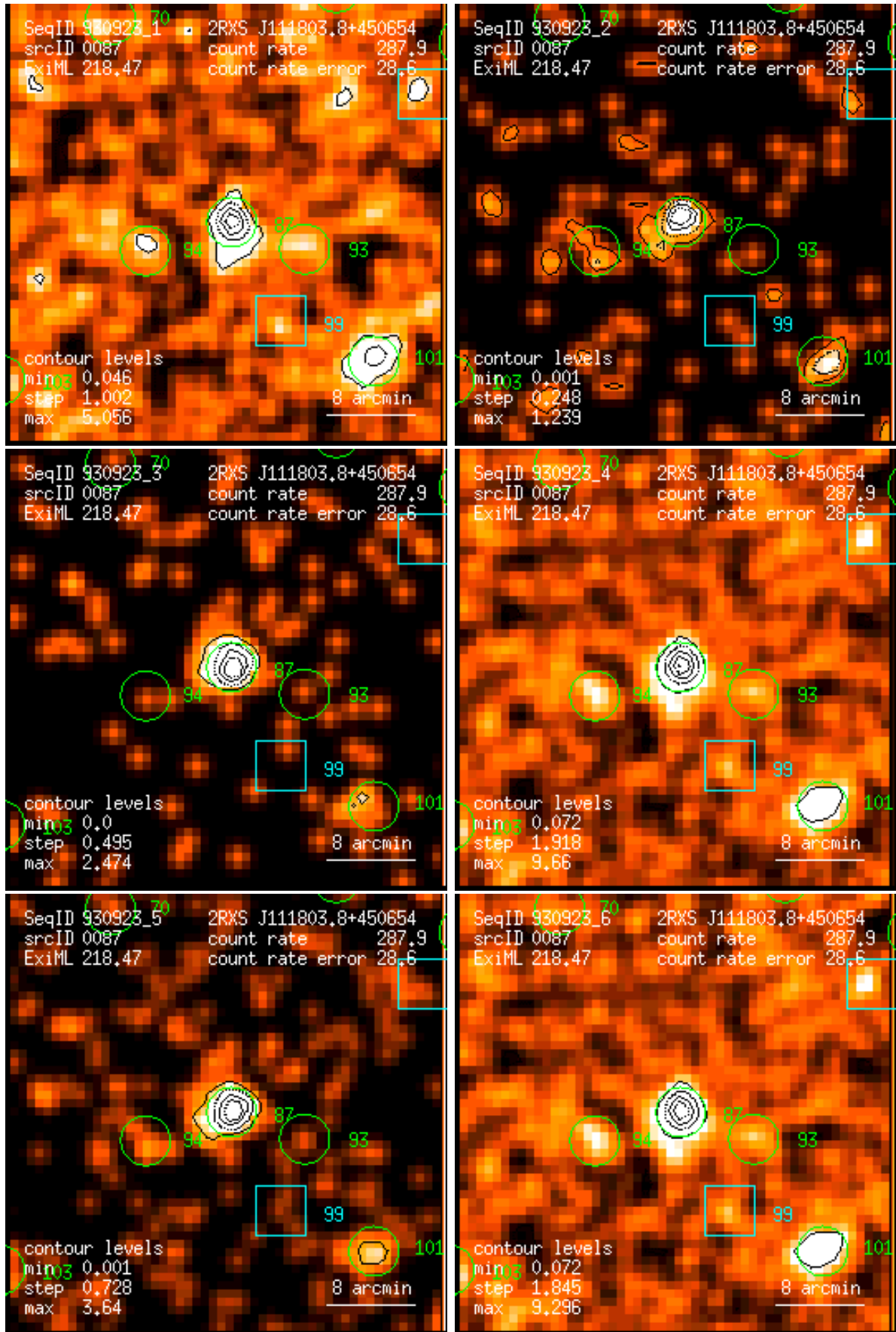
Figure 87: RASS 930923: detection 0087: band rate images, Gaussian filter: (1) PSPC channels 11 – 41, (2) 52 – 90, (3) 91 – 201, (4) 11 – 235, (5) 52 – 201, (6) 11 – 201. Broad band rates in counts/ks. Band rate contour levels in counts/ks/arcmin 2 .
