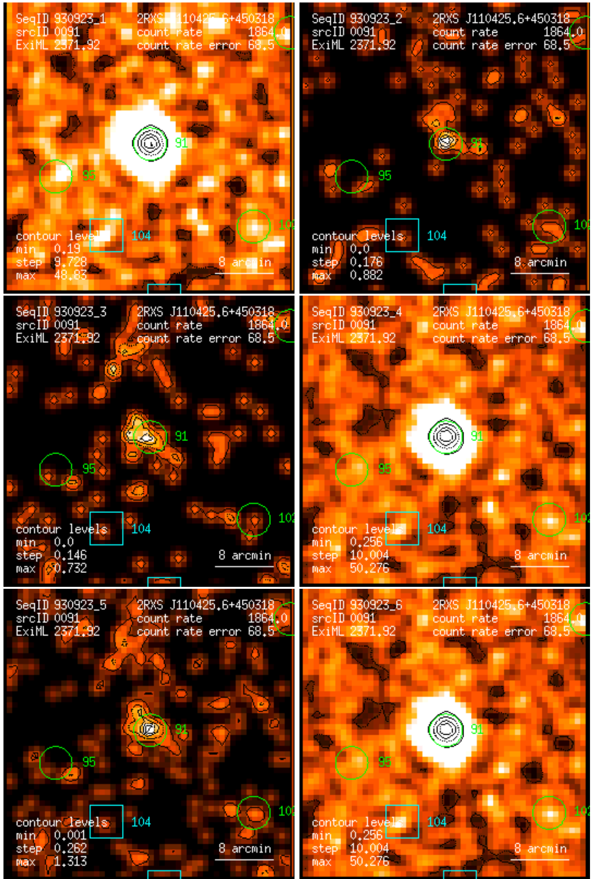
Figure 91: RASS 930923: detection 0091: band rate images, Gaussian filter: (1) PSPC channels 11 – 41, (2) 52 – 90, (3) 91 – 201, (4) 11 – 235, (5) 52 – 201, (6) 11 – 201. Broad band rates in counts/ks. Band rate contour levels in counts/ks/arcmin 2 .
