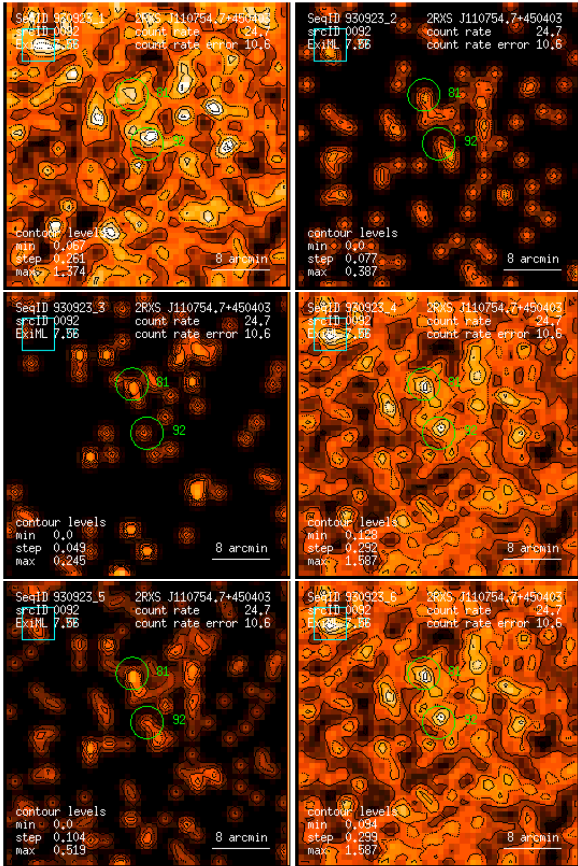
Figure 92: RASS 930923: detection 0092: band rate images, Gaussian filter: (1) PSPC channels 11 – 41, (2) 52 – 90, (3) 91 – 201, (4) 11 – 235, (5) 52 – 201, (6) 11 – 201. Broad band rates in counts/ks. Band rate contour levels in counts/ks/arcmin 2 .
