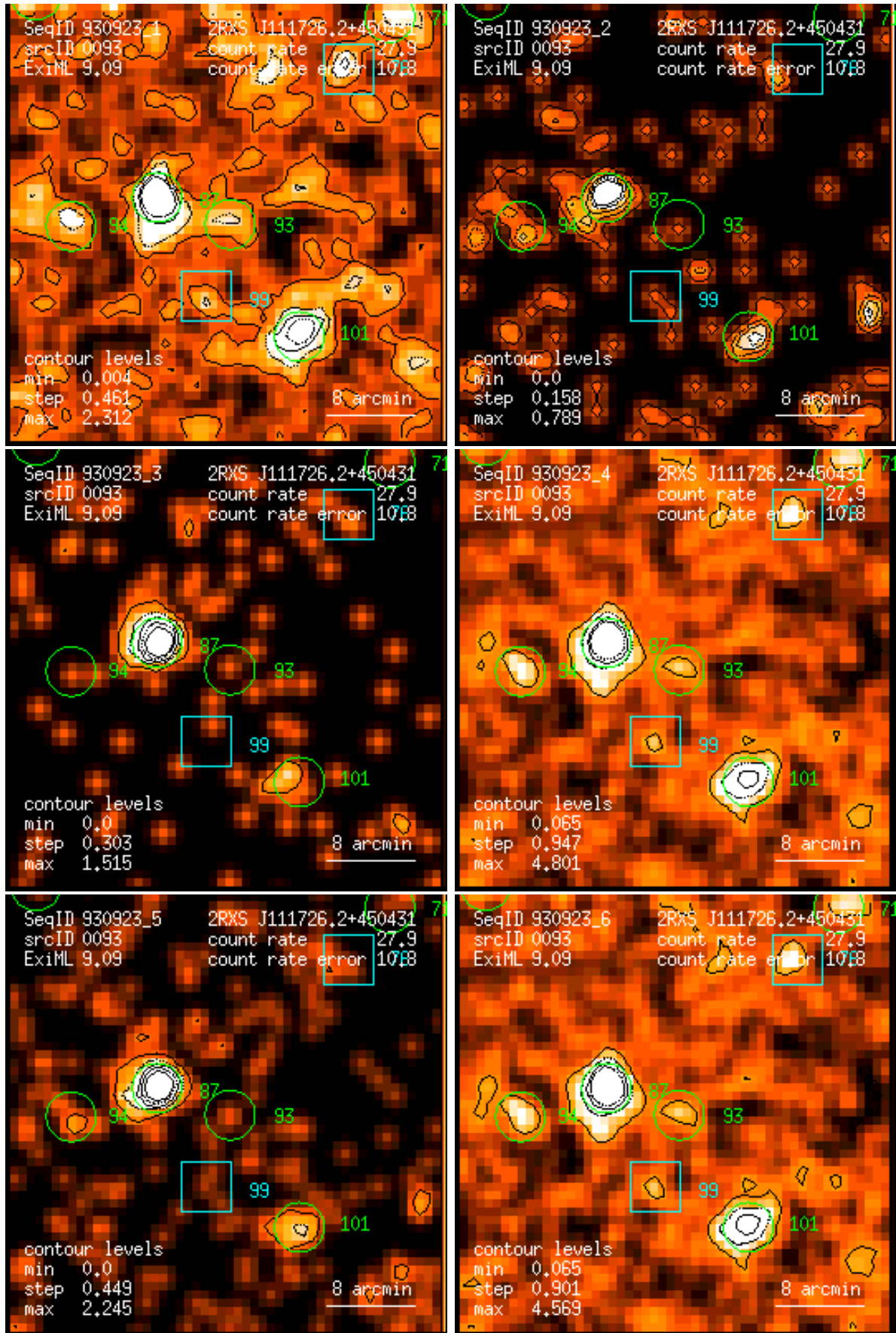
Figure 93: RASS 930923: detection 0093: band rate images, Gaussian filter: (1) PSPC channels 11 – 41, (2) 52 – 90, (3) 91 – 201, (4) 11 – 235, (5) 52 – 201, (6) 11 – 201. Broad band rates in counts/ks. Band rate contour levels in counts/ks/arcmin 2 .
