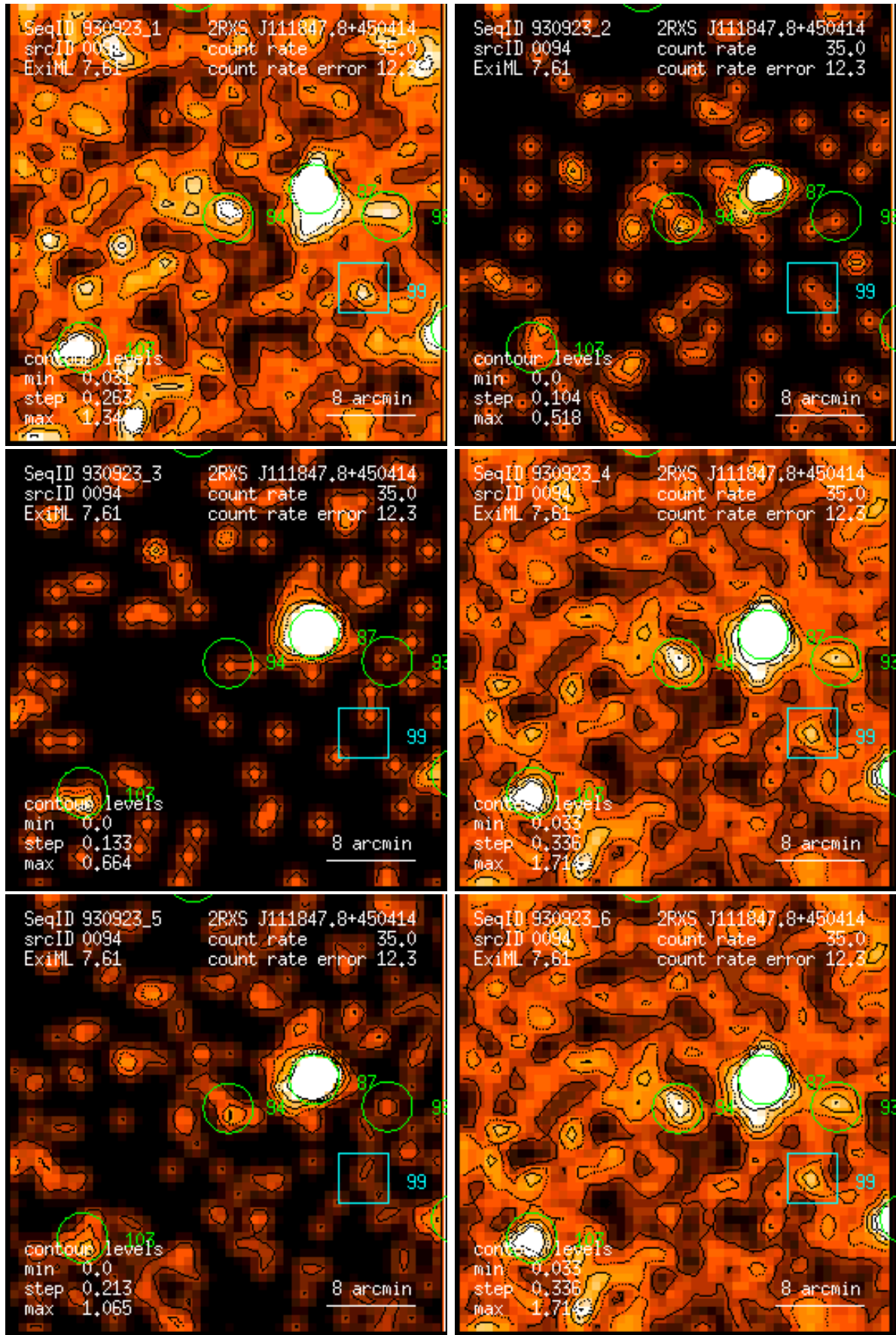
Figure 94: RASS 930923: detection 0094: band rate images, Gaussian filter: (1) PSPC channels 11 – 41, (2) 52 – 90, (3) 91 – 201, (4) 11 – 235, (5) 52 – 201, (6) 11 – 201. Broad band rates in counts/ks. Band rate contour levels in counts/ks/arcmin 2 .
