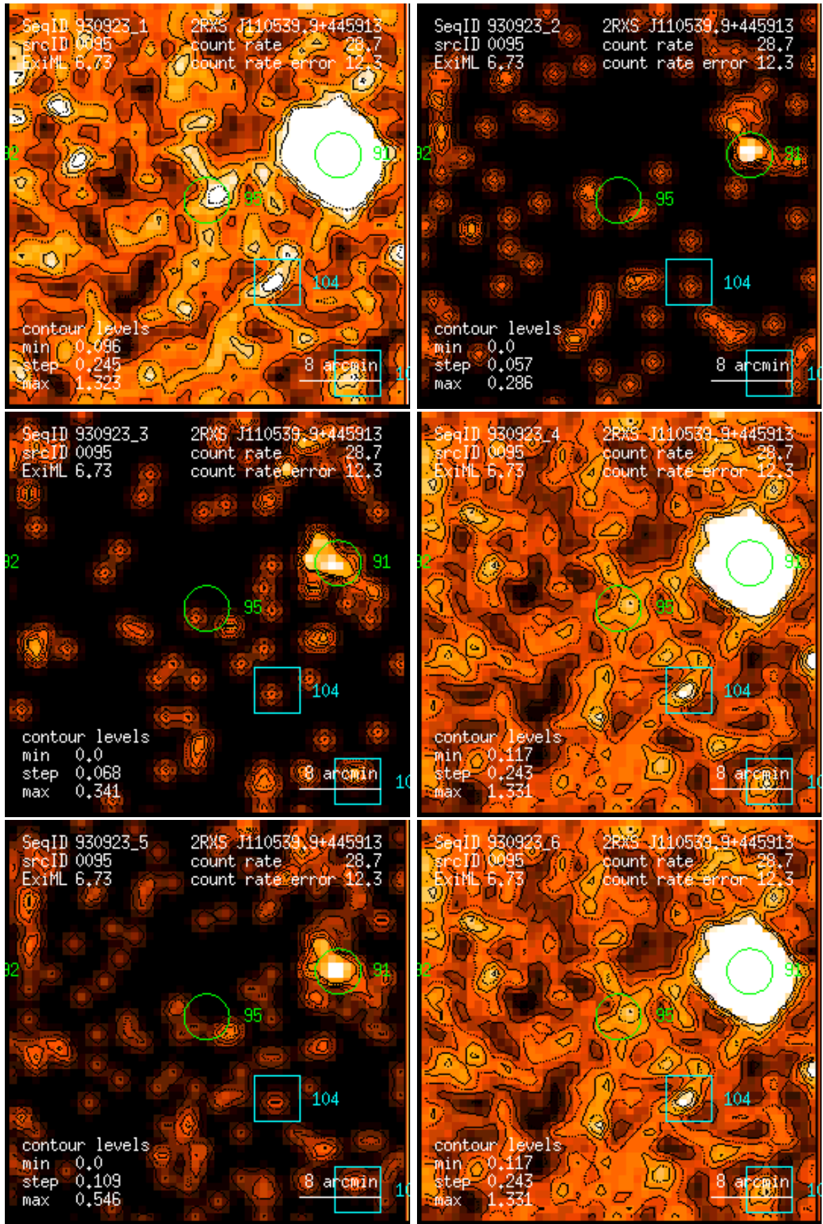
Figure 95: RASS 930923: detection 0095: band rate images, Gaussian filter: (1) PSPC channels 11 – 41, (2) 52 – 90, (3) 91 – 201, (4) 11 – 235, (5) 52 – 201, (6) 11 – 201. Broad band rates in counts/ks. Band rate contour levels in counts/ks/arcmin 2 .
