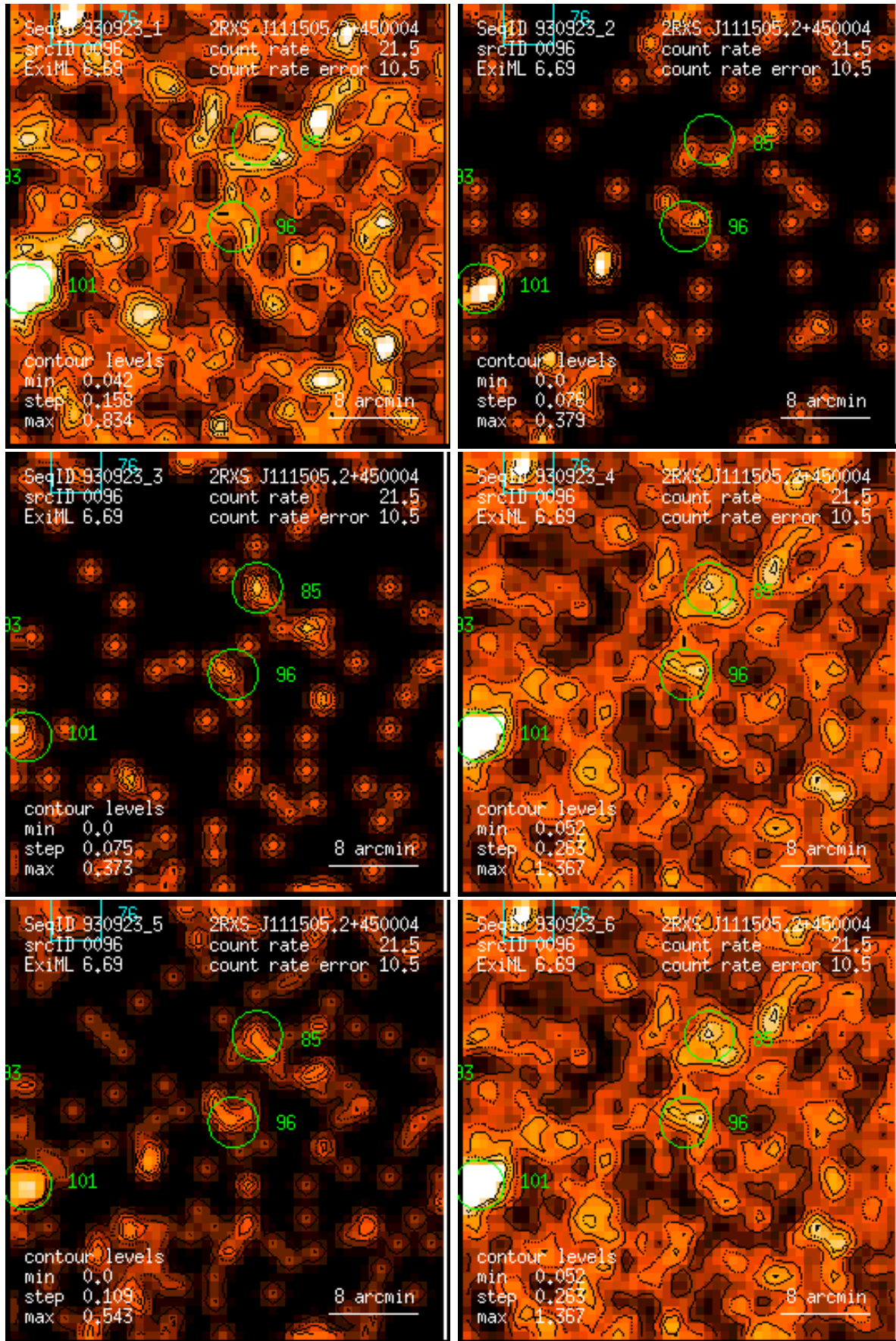
Figure 96: RASS 930923: detection 0096: band rate images, Gaussian filter: (1) PSPC channels 11 – 41, (2) 52 – 90, (3) 91 – 201, (4) 11 – 235, (5) 52 – 201, (6) 11 – 201. Broad band rates in counts/ks. Band rate contour levels in counts/ks/arcmin 2 .
