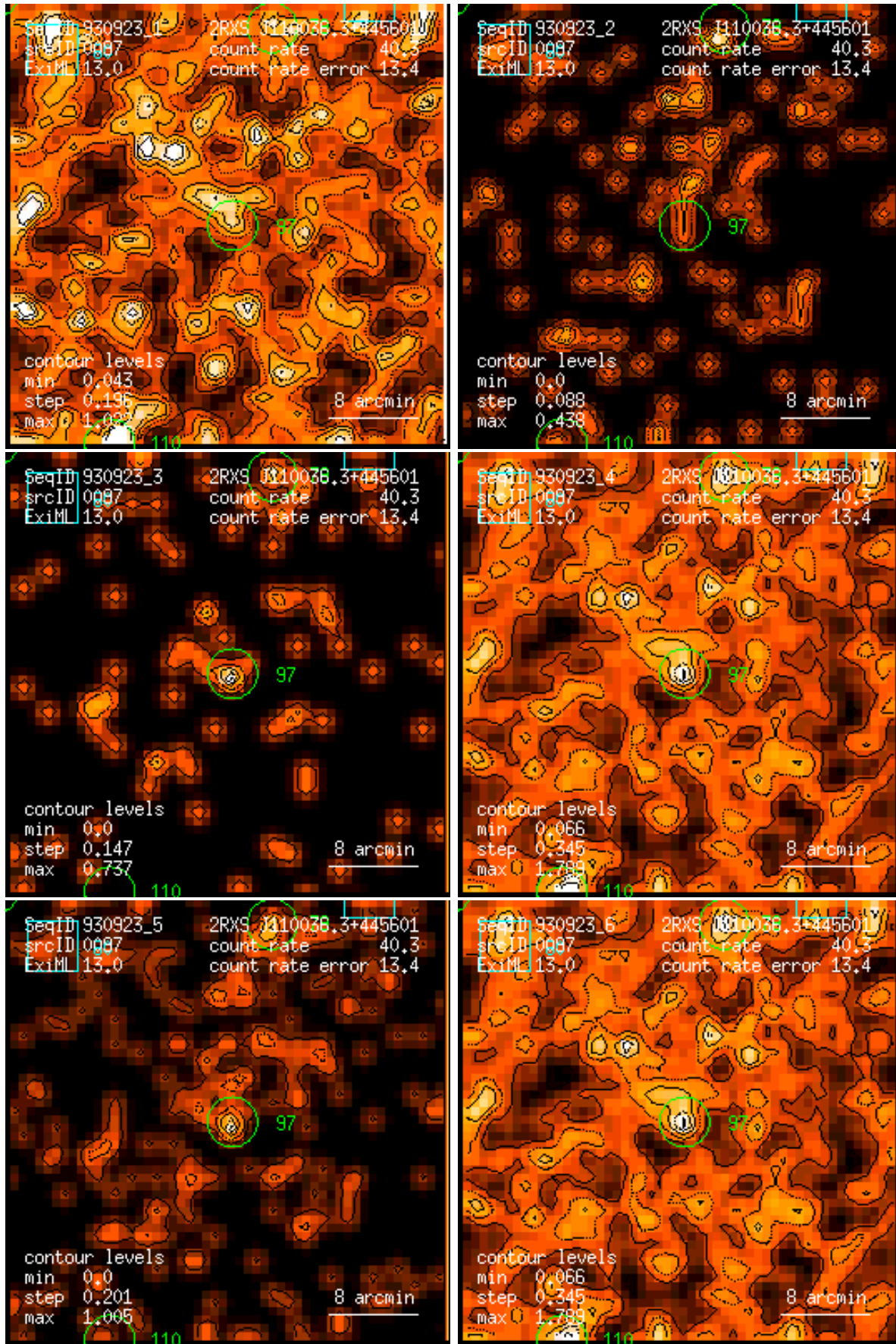
Figure 97: RASS 930923: detection 0097: band rate images, Gaussian filter: (1) PSPC channels 11 – 41, (2) 52 – 90, (3) 91 – 201, (4) 11 – 235, (5) 52 – 201, (6) 11 – 201. Broad band rates in counts/ks. Band rate contour levels in counts/ks/arcmin 2 .
