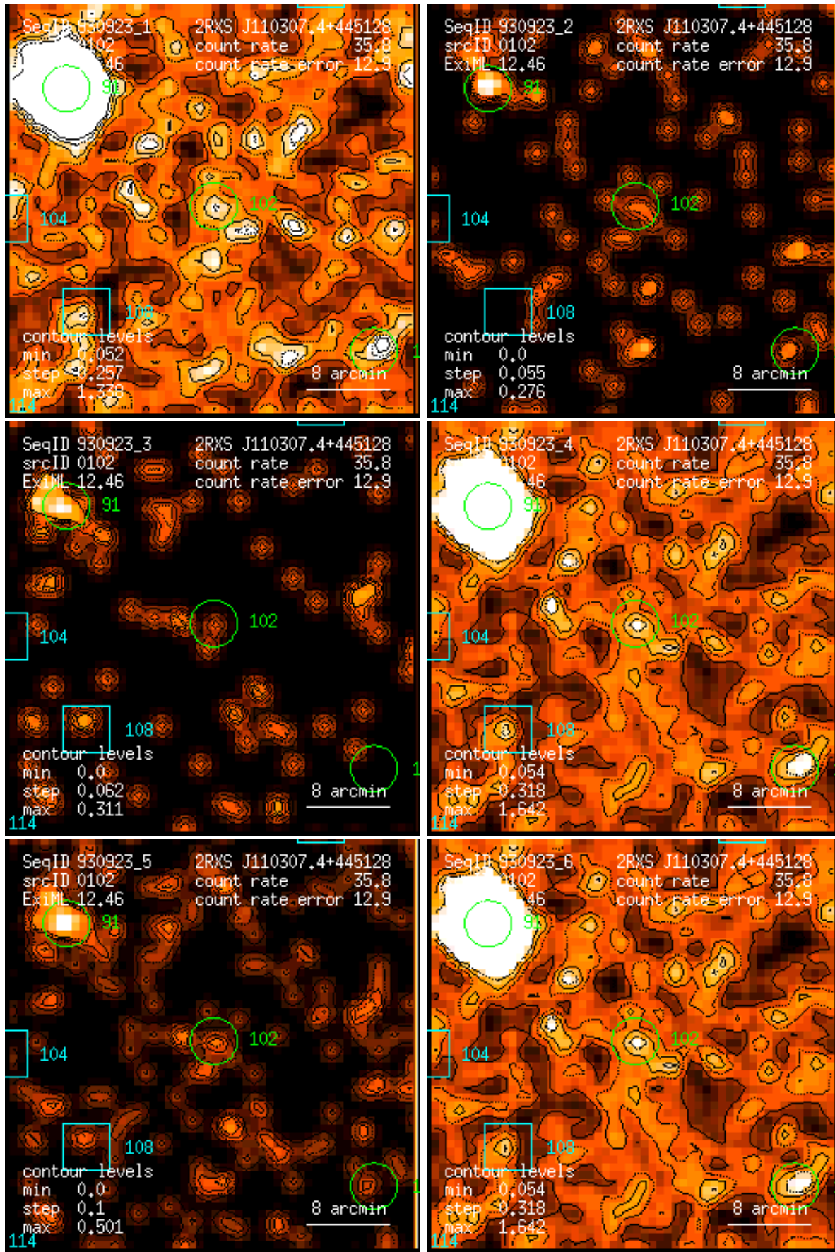
Figure 102: RASS 930923: detection 0102: band rate images, Gaussian filter: (1) PSPC channels 11 – 41, (2) 52 – 90, (3) 91 – 201, (4) 11 – 235, (5) 52 – 201, (6) 11 – 201. Broad band rates in counts/ks. Band rate contour levels in counts/ks/arcmin 2 .
