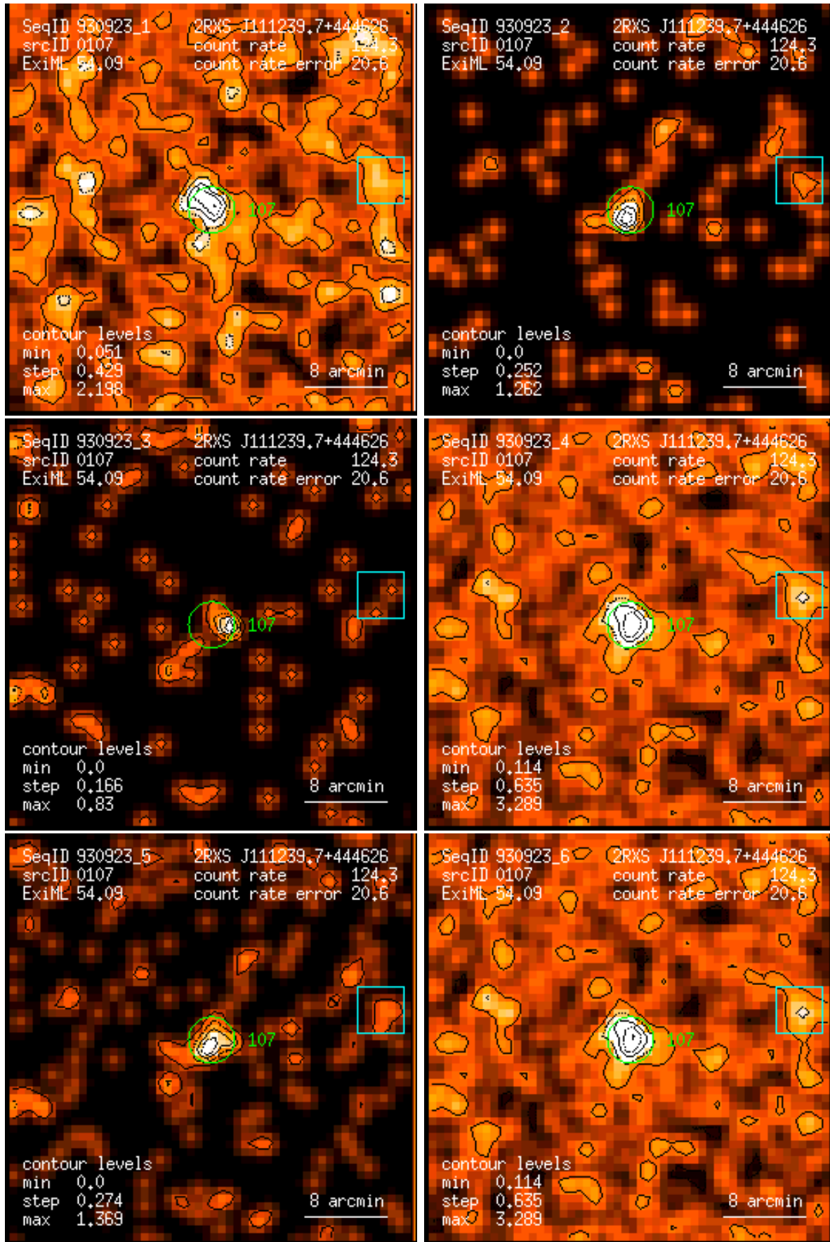
Figure 107: RASS 930923: detection 0107: band rate images, Gaussian filter: (1) PSPC channels 11 – 41, (2) 52 – 90, (3) 91 – 201, (4) 11 – 235, (5) 52 – 201, (6) 11 – 201. Broad band rates in counts/ks. Band rate contour levels in counts/ks/arcmin 2 .
