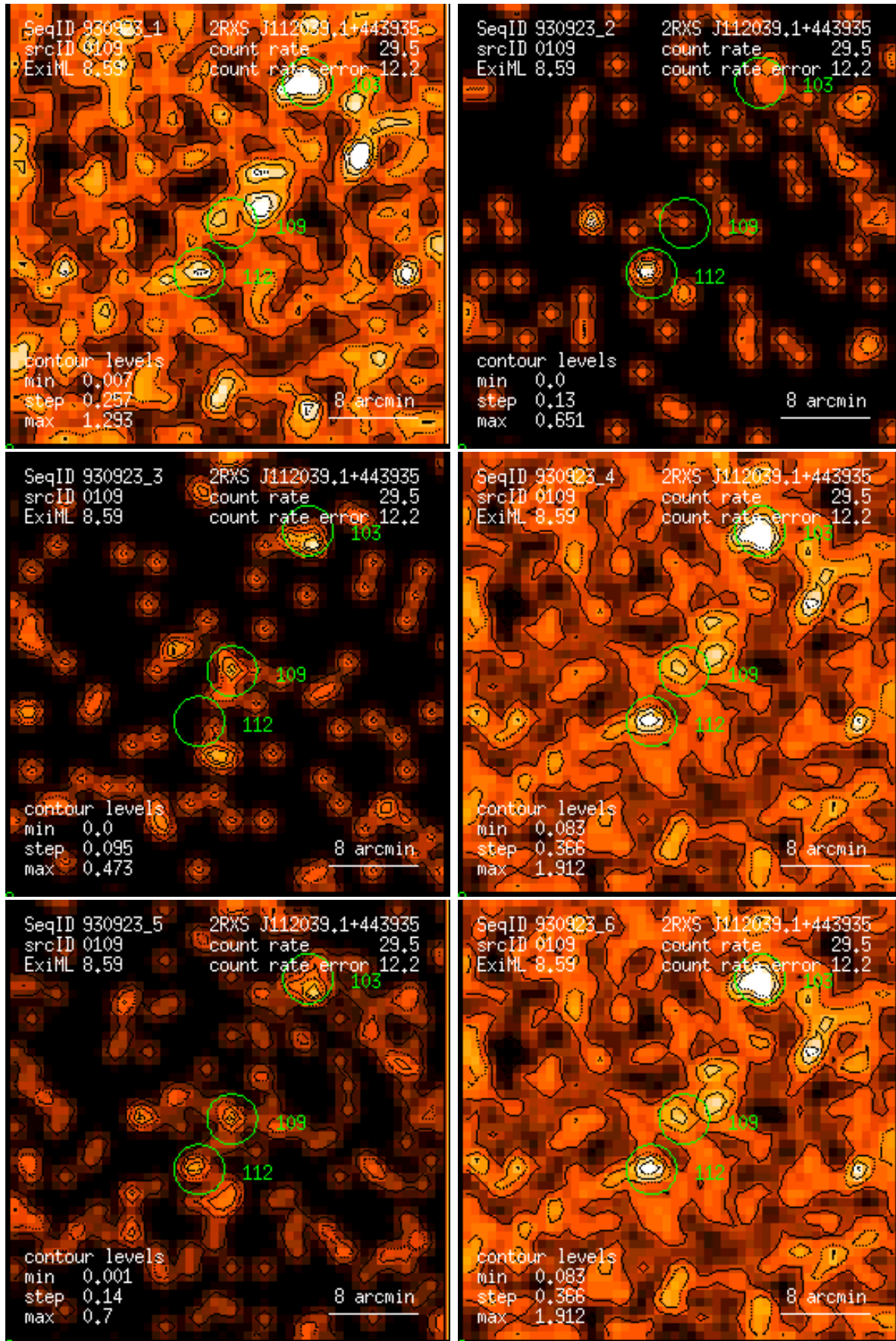
Figure 109: RASS 930923: detection 0109: band rate images, Gaussian filter: (1) PSPC channels 11 – 41, (2) 52 – 90, (3) 91 – 201, (4) 11 – 235, (5) 52 – 201, (6) 11 – 201. Broad band rates in counts/ks. Band rate contour levels in counts/ks/arcmin 2 .
