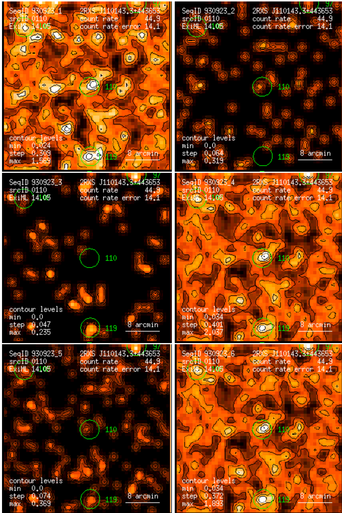
Figure 110: RASS 930923: detection 0110: band rate images, Gaussian filter: (1) PSPC channels 11 – 41, (2) 52 – 90, (3) 91 – 201, (4) 11 – 235, (5) 52 – 201, (6) 11 – 201. Broad band rates in counts/ks. Band rate contour levels in counts/ks/arcmin 2 .
