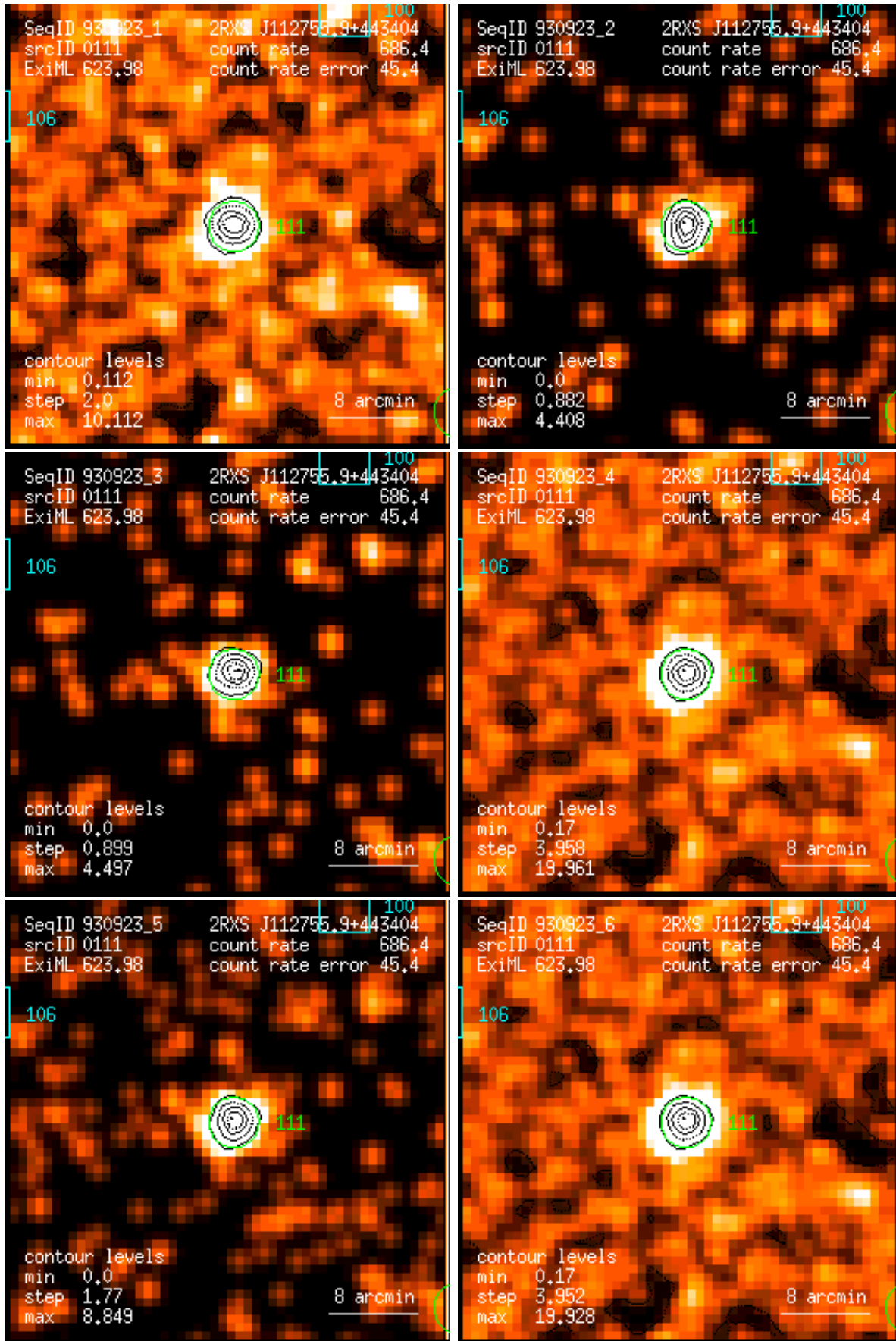
Figure 111: RASS 930923: detection 0111: band rate images, Gaussian filter: (1) PSPC channels 11 – 41, (2) 52 – 90, (3) 91 – 201, (4) 11 – 235, (5) 52 – 201, (6) 11 – 201. Broad band rates in counts/ks. Band rate contour levels in counts/ks/arcmin 2 .
