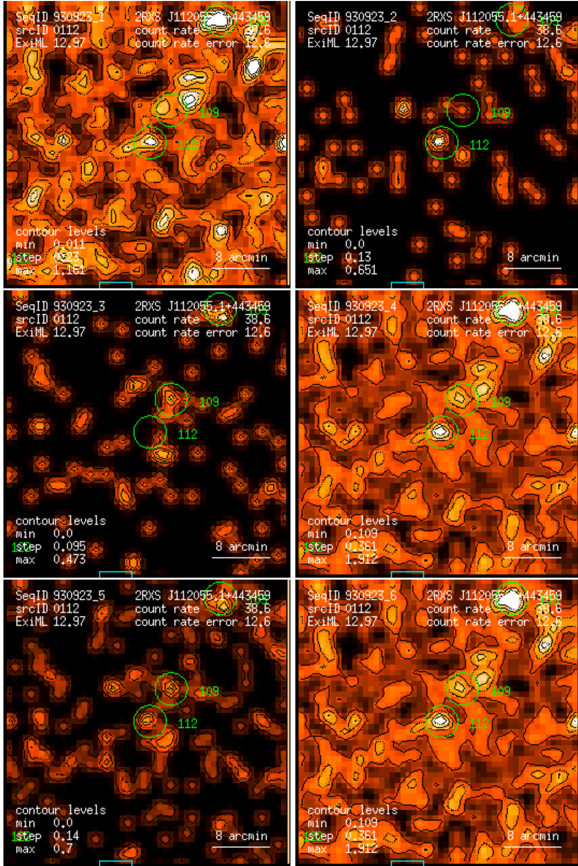
Figure 112: RASS 930923: detection 0112: band rate images, Gaussian filter: (1) PSPC channels 11 – 41, (2) 52 – 90, (3) 91 – 201, (4) 11 – 235, (5) 52 – 201, (6) 11 – 201. Broad band rates in counts/ks. Band rate contour levels in counts/ks/arcmin 2 .
