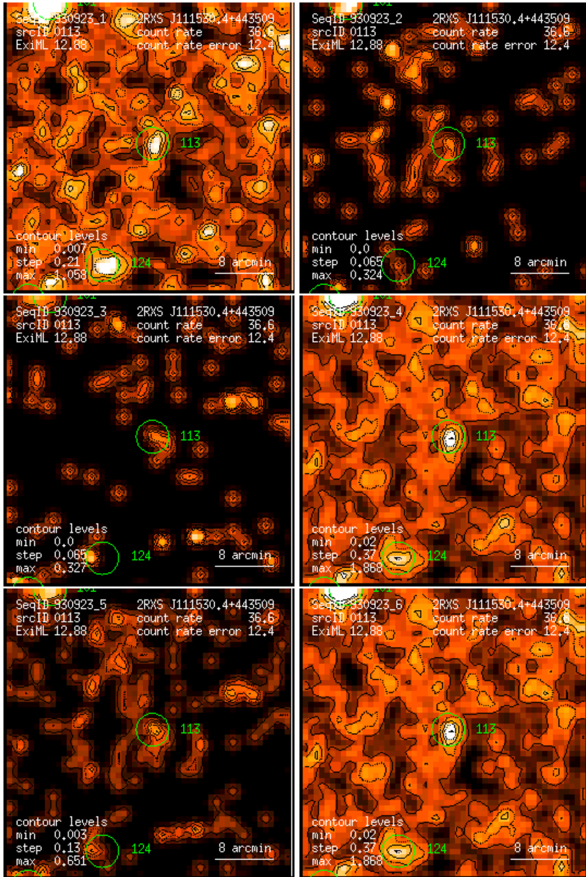
Figure 113: RASS 930923: detection 0113: band rate images, Gaussian filter: (1) PSPC channels 11 – 41, (2) 52 – 90, (3) 91 – 201, (4) 11 – 235, (5) 52 – 201, (6) 11 – 201. Broad band rates in counts/ks. Band rate contour levels in counts/ks/arcmin 2 .
