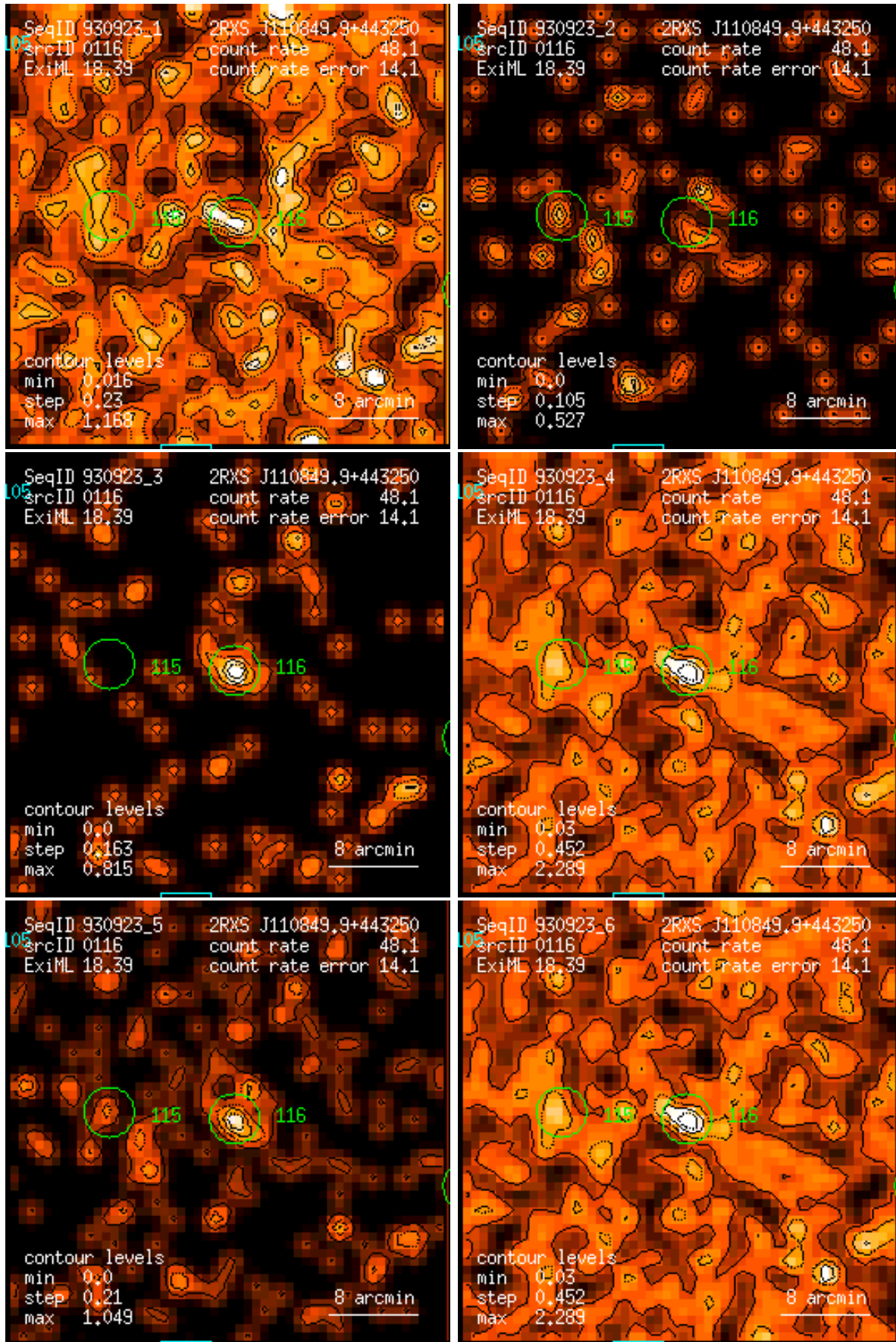
Figure 116: RASS 930923: detection 0116: band rate images, Gaussian filter: (1) PSPC channels 11 – 41, (2) 52 – 90, (3) 91 – 201, (4) 11 – 235, (5) 52 – 201, (6) 11 – 201. Broad band rates in counts/ks. Band rate contour levels in counts/ks/arcmin 2 .
