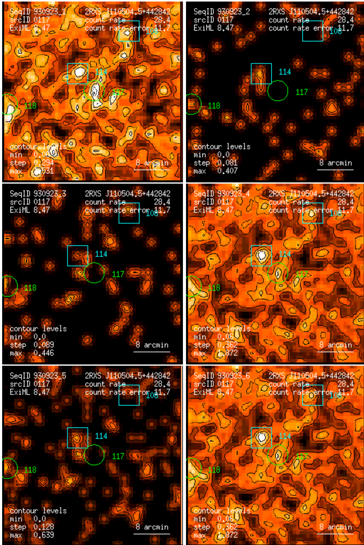
Figure 117: RASS 930923: detection 0117: band rate images, Gaussian filter: (1) PSPC channels 11 – 41, (2) 52 – 90, (3) 91 – 201, (4) 11 – 235, (5) 52 – 201, (6) 11 – 201. Broad band rates in counts/ks. Band rate contour levels in counts/ks/arcmin 2 .
