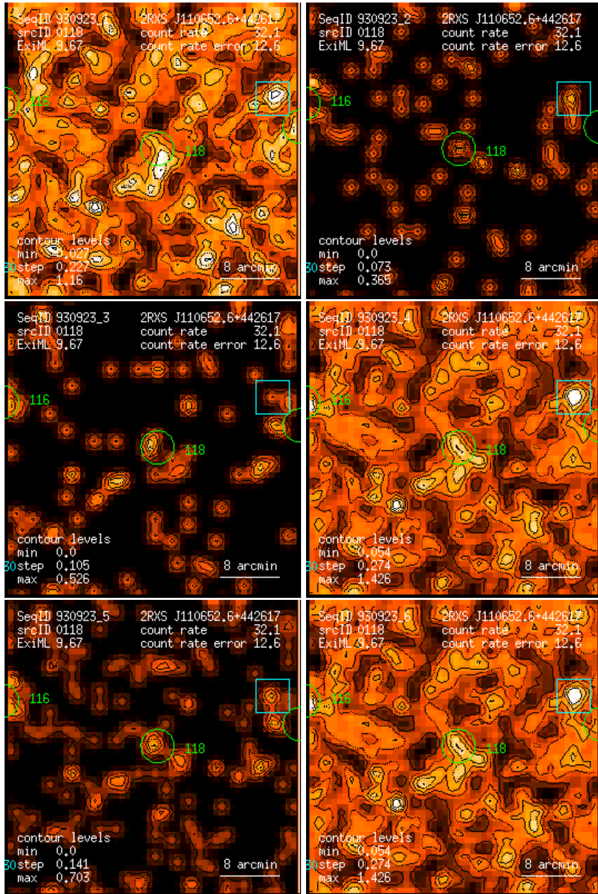
Figure 118: RASS 930923: detection 0118: band rate images, Gaussian filter: (1) PSPC channels 11 – 41, (2) 52 – 90, (3) 91 – 201, (4) 11 – 235, (5) 52 – 201, (6) 11 – 201. Broad band rates in counts/ks. Band rate contour levels in counts/ks/arcmin 2 .
