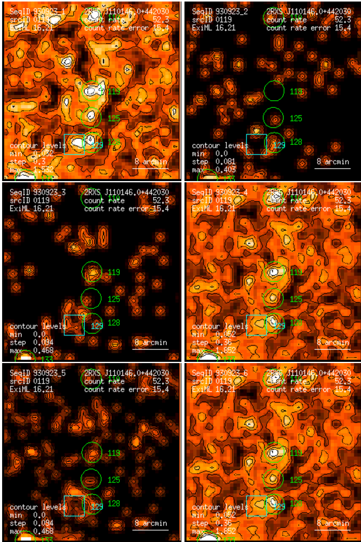
Figure 119: RASS 930923: detection 0119: band rate images, Gaussian filter: (1) PSPC channels 11 – 41, (2) 52 – 90, (3) 91 – 201, (4) 11 – 235, (5) 52 – 201, (6) 11 – 201. Broad band rates in counts/ks. Band rate contour levels in counts/ks/arcmin 2 .
