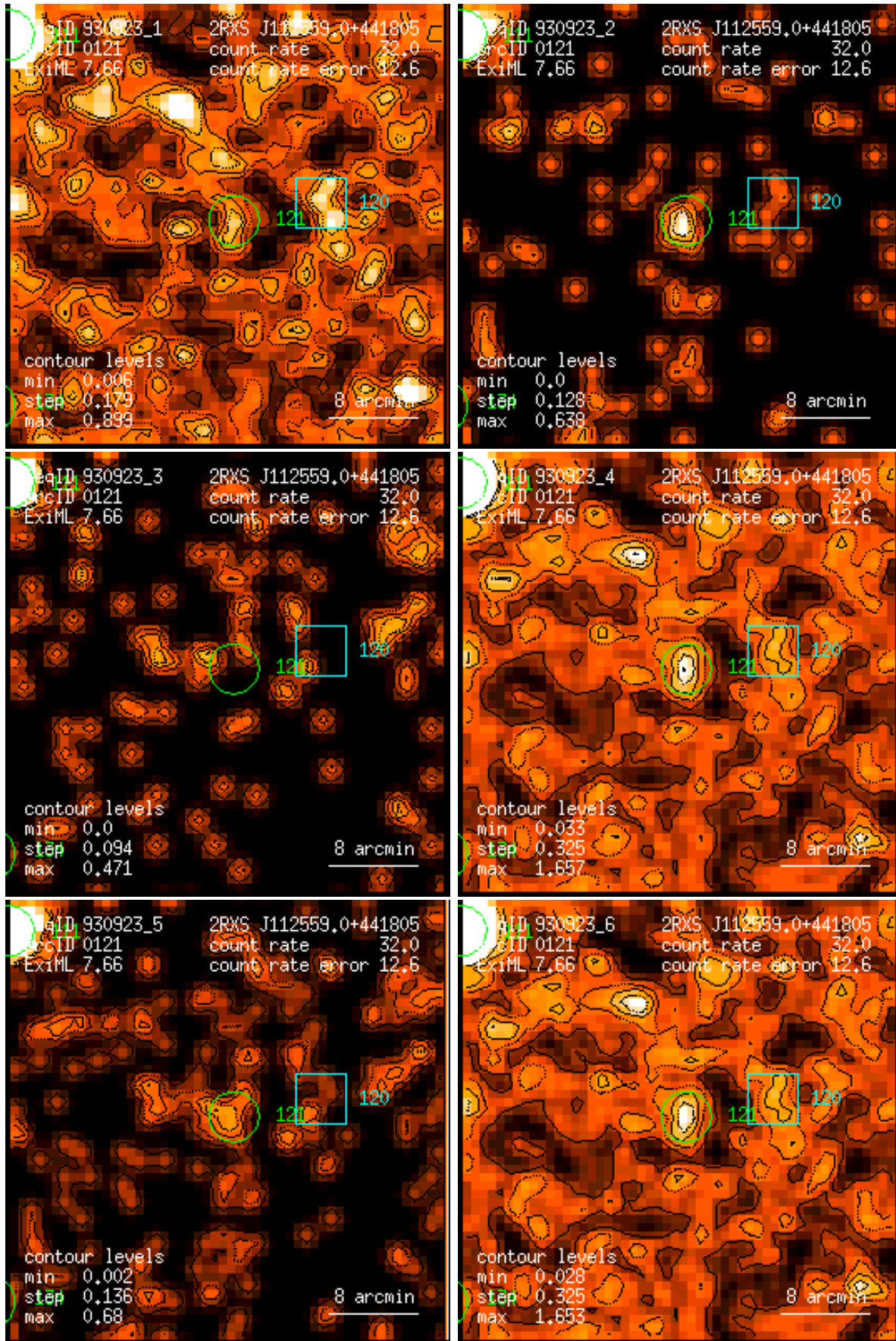
Figure 121: RASS 930923: detection 0121: band rate images, Gaussian filter: (1) PSPC channels 11 – 41, (2) 52 – 90, (3) 91 – 201, (4) 11 – 235, (5) 52 – 201, (6) 11 – 201. Broad band rates in counts/ks. Band rate contour levels in counts/ks/arcmin 2 .
