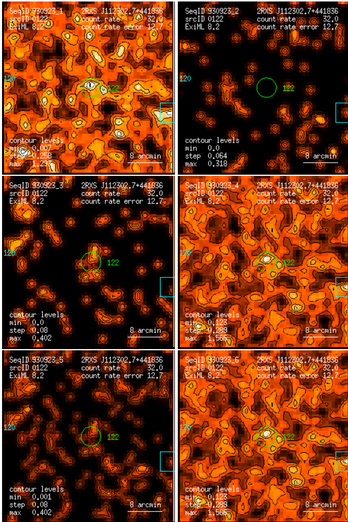
Figure 122: RASS 930923: detection 0122: band rate images, Gaussian filter: (1) PSPC channels 11 – 41, (2) 52 – 90, (3) 91 – 201, (4) 11 – 235, (5) 52 – 201, (6) 11 – 201. Broad band rates in counts/ks. Band rate contour levels in counts/ks/arcmin 2 .
