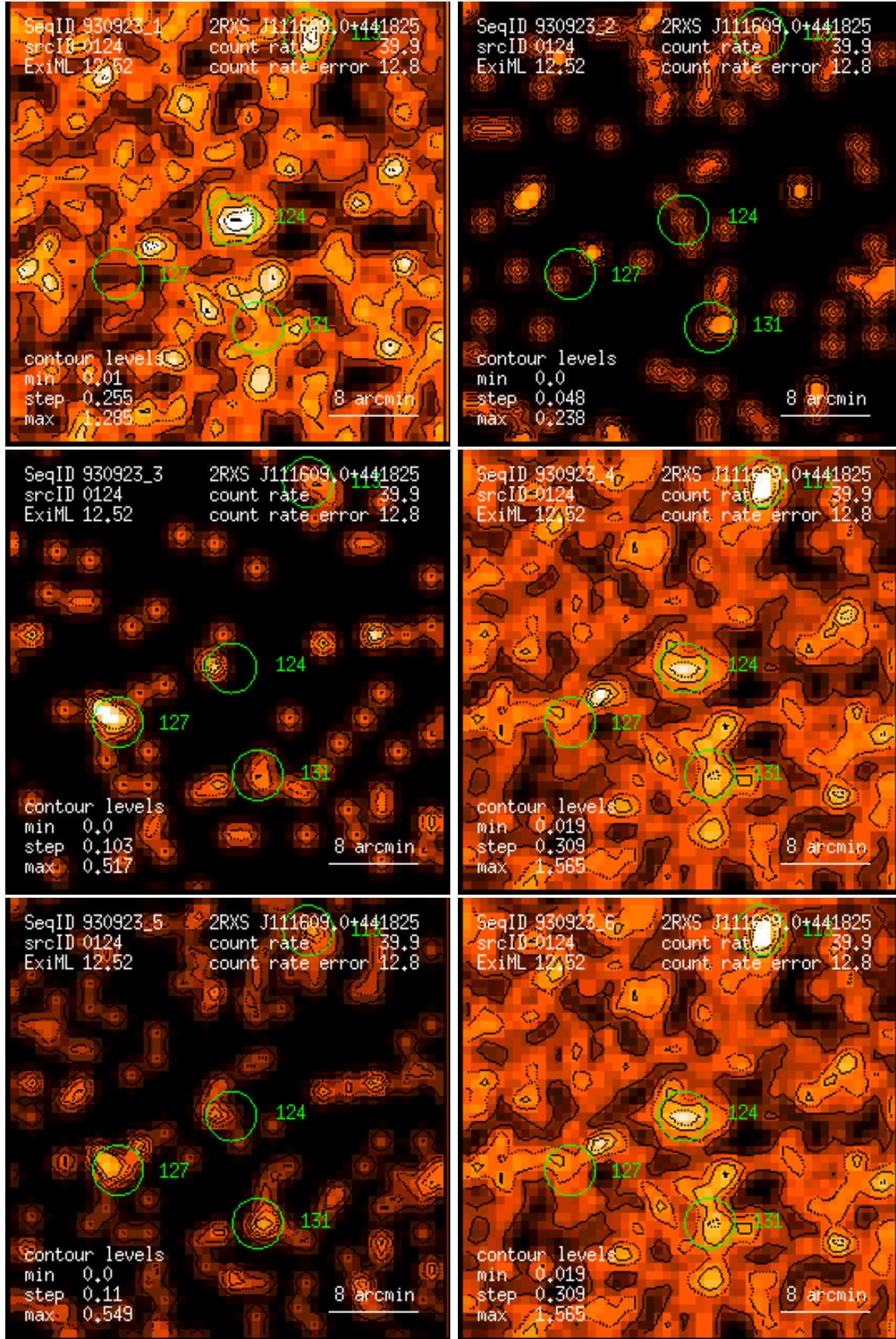
Figure 124: RASS 930923: detection 0124: band rate images, Gaussian filter: (1) PSPC channels 11 – 41, (2) 52 – 90, (3) 91 – 201, (4) 11 – 235, (5) 52 – 201, (6) 11 – 201. Broad band rates in counts/ks. Band rate contour levels in counts/ks/arcmin 2 .
