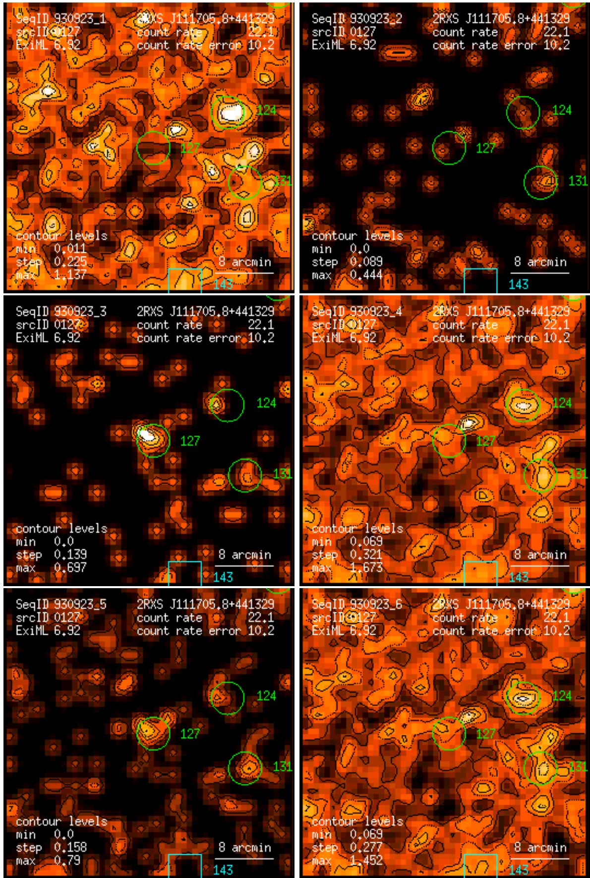
Figure 127: RASS 930923: detection 0127: band rate images, Gaussian filter: (1) PSPC channels 11 – 41, (2) 52 – 90, (3) 91 – 201, (4) 11 – 235, (5) 52 – 201, (6) 11 – 201. Broad band rates in counts/ks. Band rate contour levels in counts/ks/arcmin 2 .
