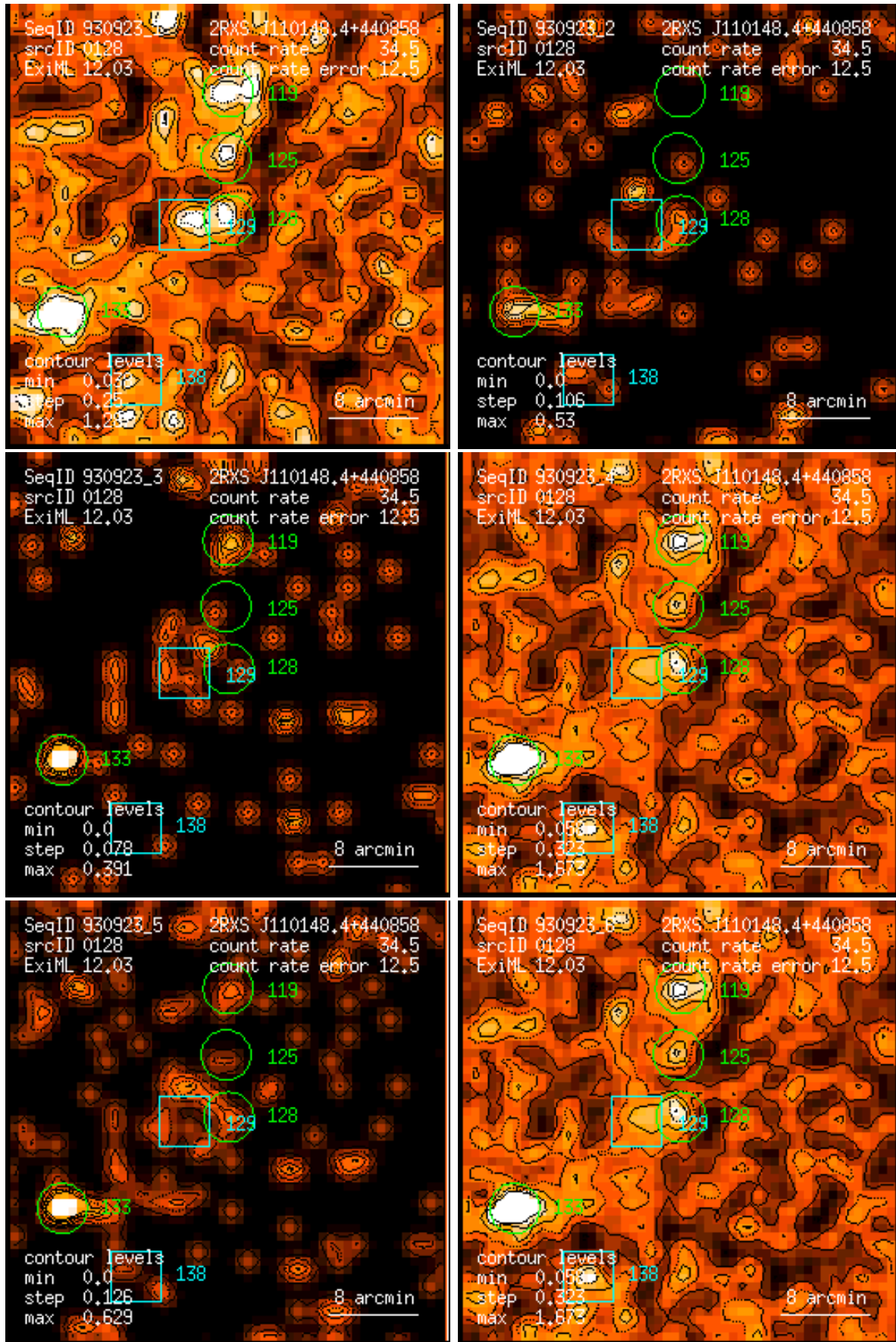
Figure 128: RASS 930923: detection 0128: band rate images, Gaussian filter: (1) PSPC channels 11 – 41, (2) 52 – 90, (3) 91 – 201, (4) 11 – 235, (5) 52 – 201, (6) 11 – 201. Broad band rates in counts/ks. Band rate contour levels in counts/ks/arcmin 2 .
