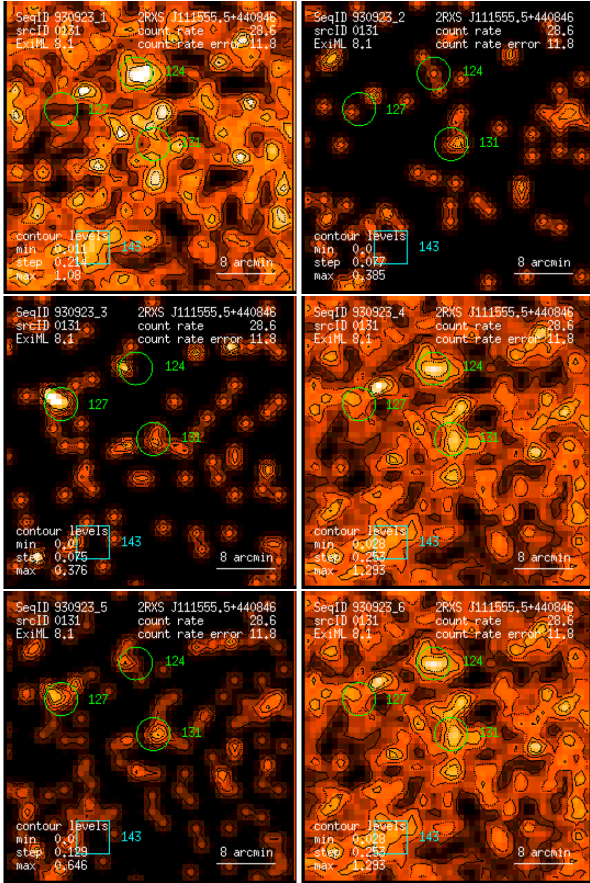
Figure 131: RASS 930923: detection 0131: band rate images, Gaussian filter: (1) PSPC channels 11 – 41, (2) 52 – 90, (3) 91 – 201, (4) 11 – 235, (5) 52 – 201, (6) 11 – 201. Broad band rates in counts/ks. Band rate contour levels in counts/ks/arcmin 2 .
