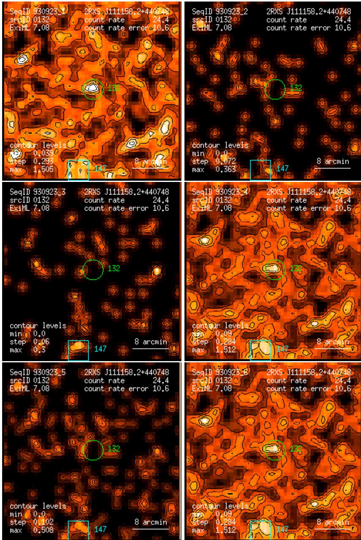
Figure 132: RASS 930923: detection 0132: band rate images, Gaussian filter: (1) PSPC channels 11 – 41, (2) 52 – 90, (3) 91 – 201, (4) 11 – 235, (5) 52 – 201, (6) 11 – 201. Broad band rates in counts/ks. Band rate contour levels in counts/ks/arcmin 2 .
