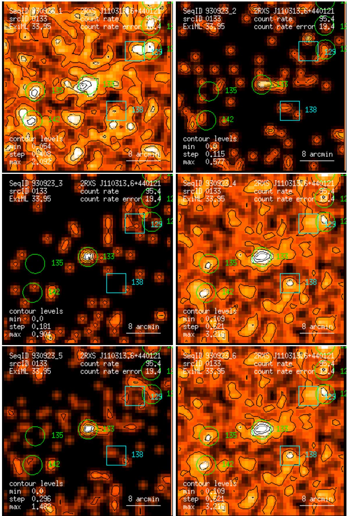
Figure 133: RASS 930923: detection 0133: band rate images, Gaussian filter: (1) PSPC channels 11 – 41, (2) 52 – 90, (3) 91 – 201, (4) 11 – 235, (5) 52 – 201, (6) 11 – 201. Broad band rates in counts/ks. Band rate contour levels in counts/ks/arcmin 2 .
