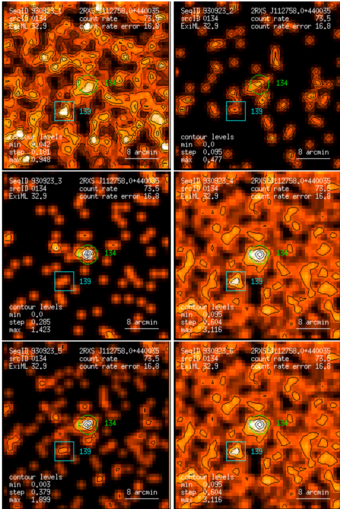
Figure 134: RASS 930923: detection 0134: band rate images, Gaussian filter: (1) PSPC channels 11 – 41, (2) 52 – 90, (3) 91 – 201, (4) 11 – 235, (5) 52 – 201, (6) 11 – 201. Broad band rates in counts/ks. Band rate contour levels in counts/ks/arcmin 2 .
