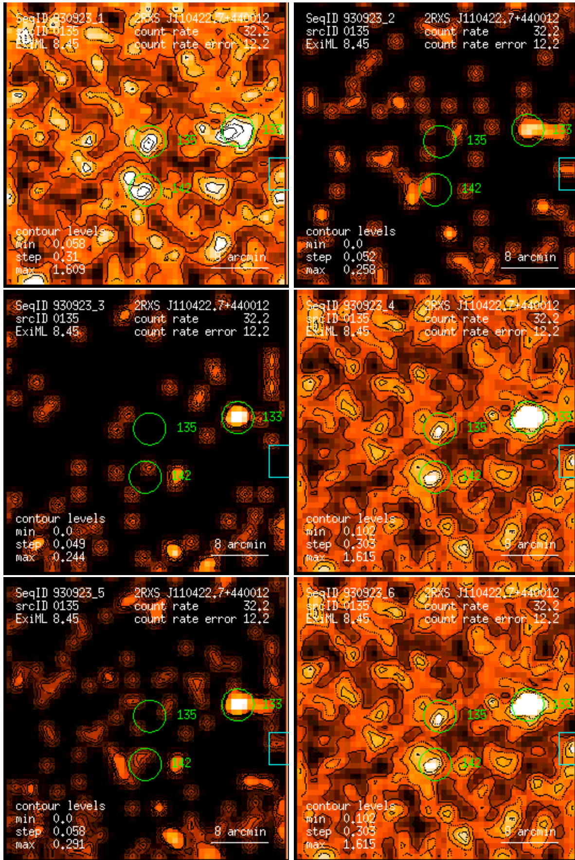
Figure 135: RASS 930923: detection 0135: band rate images, Gaussian filter: (1) PSPC channels 11 – 41, (2) 52 – 90, (3) 91 – 201, (4) 11 – 235, (5) 52 – 201, (6) 11 – 201. Broad band rates in counts/ks. Band rate contour levels in counts/ks/arcmin 2 .
