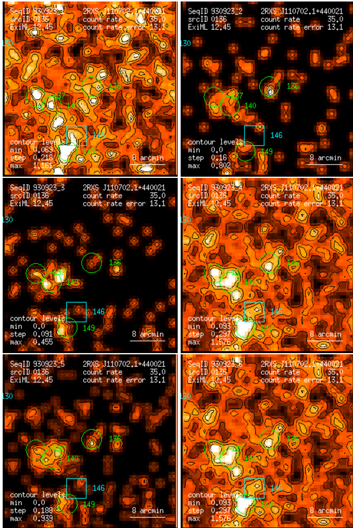
Figure 136: RASS 930923: detection 0136: band rate images, Gaussian filter: (1) PSPC channels 11 – 41, (2) 52 – 90, (3) 91 – 201, (4) 11 – 235, (5) 52 – 201, (6) 11 – 201. Broad band rates in counts/ks. Band rate contour levels in counts/ks/arcmin 2 .
