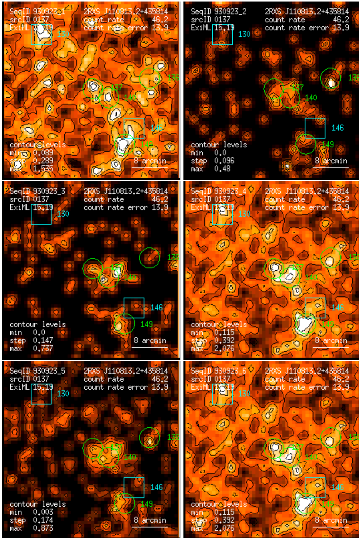
Figure 137: RASS 930923: detection 0137: band rate images, Gaussian filter: (1) PSPC channels 11 – 41, (2) 52 – 90, (3) 91 – 201, (4) 11 – 235, (5) 52 – 201, (6) 11 – 201. Broad band rates in counts/ks. Band rate contour levels in counts/ks/arcmin 2 .
