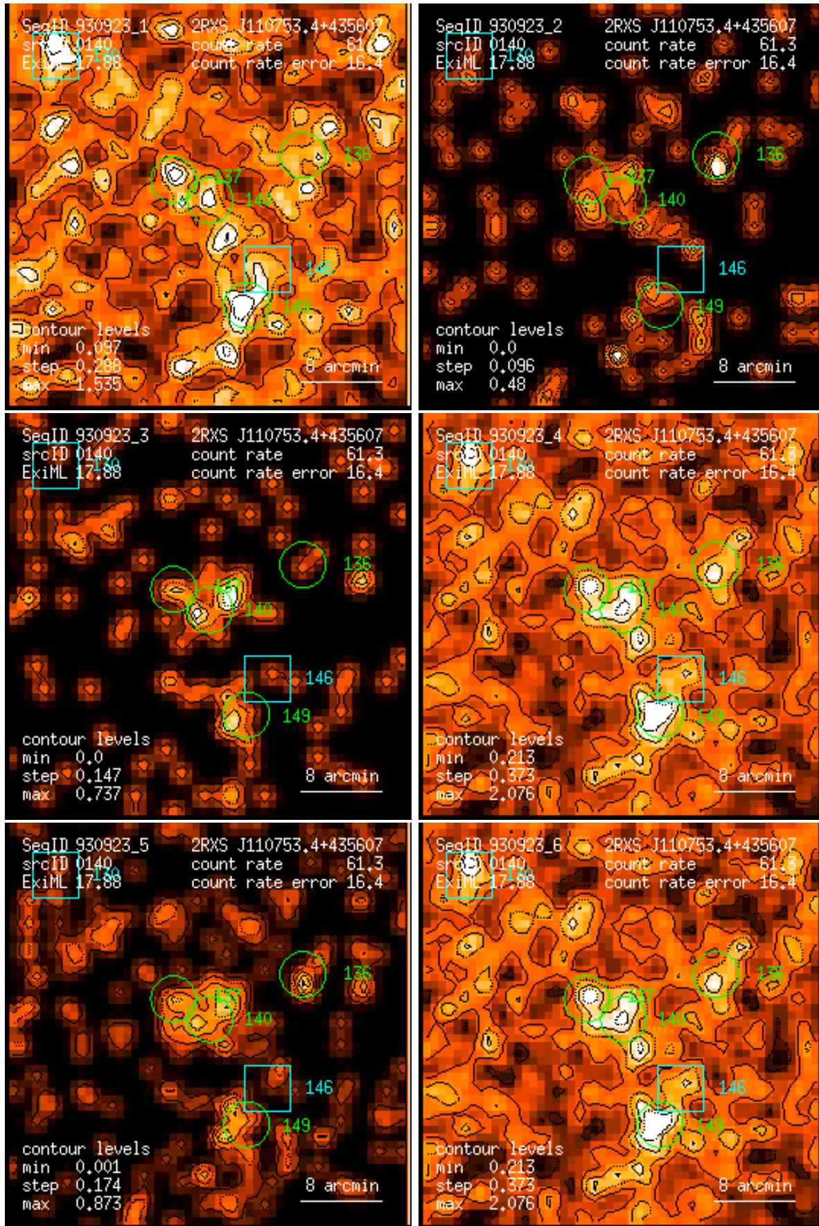
Figure 140: RASS 930923: detection 0140: band rate images, Gaussian filter: (1) PSPC channels 11 – 41, (2) 52 – 90, (3) 91 – 201, (4) 11 – 235, (5) 52 – 201, (6) 11 – 201. Broad band rates in counts/ks. Band rate contour levels in counts/ks/arcmin 2 .
