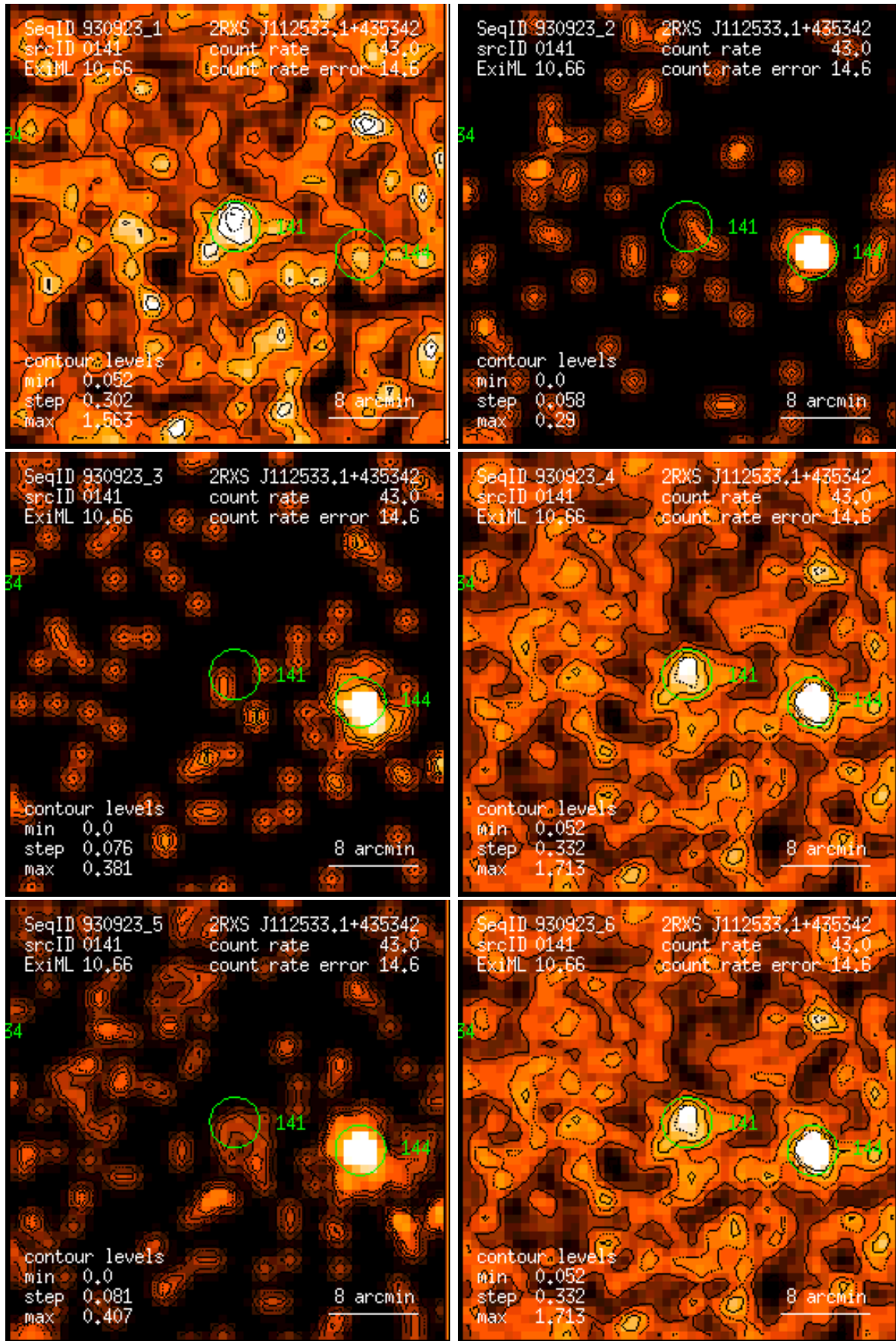
Figure 141: RASS 930923: detection 0141: band rate images, Gaussian filter: (1) PSPC channels 11 – 41, (2) 52 – 90, (3) 91 – 201, (4) 11 – 235, (5) 52 – 201, (6) 11 – 201. Broad band rates in counts/ks. Band rate contour levels in counts/ks/arcmin 2 .
