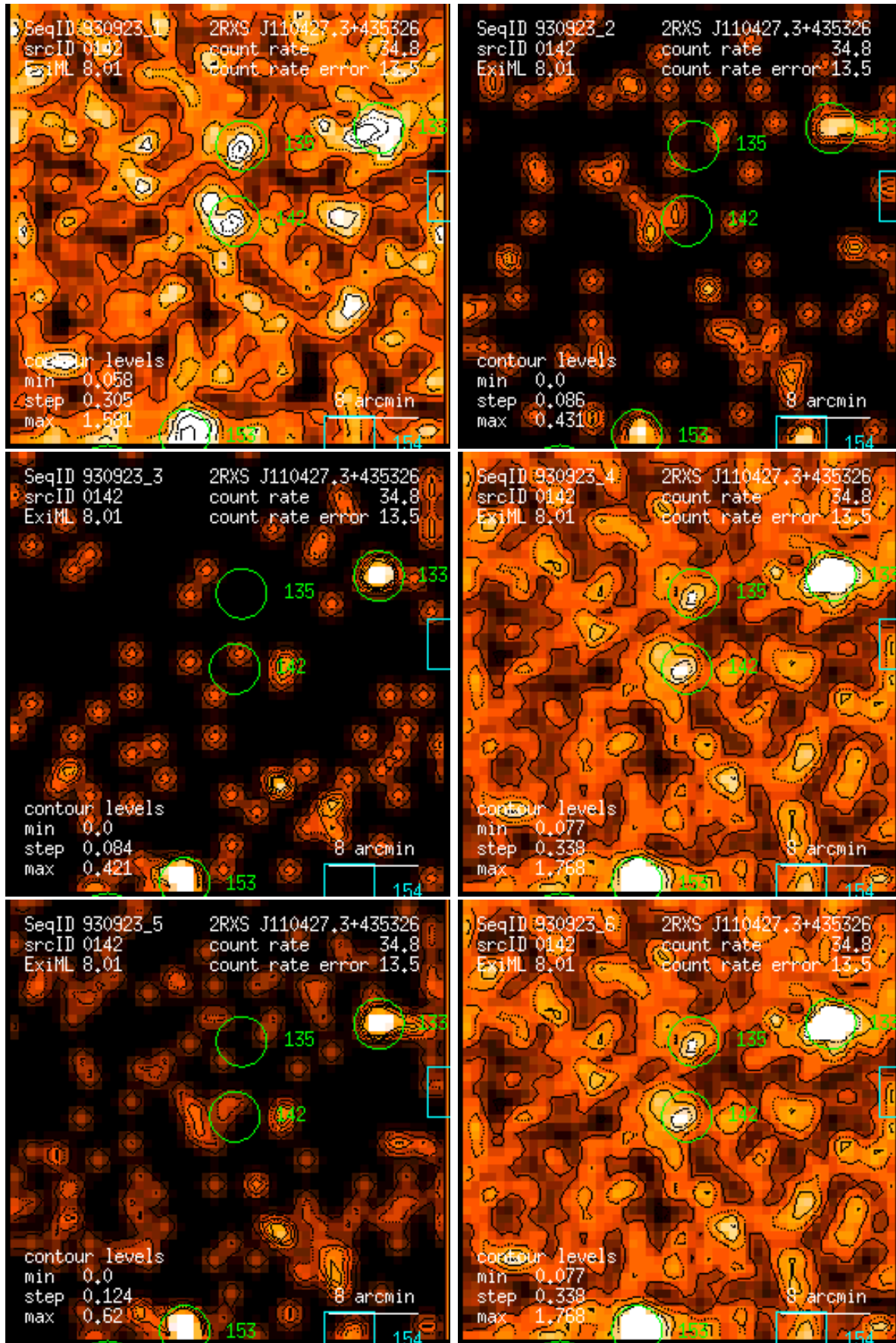
Figure 142: RASS 930923: detection 0142: band rate images, Gaussian filter: (1) PSPC channels 11 – 41, (2) 52 – 90, (3) 91 – 201, (4) 11 – 235, (5) 52 – 201, (6) 11 – 201. Broad band rates in counts/ks. Band rate contour levels in counts/ks/arcmin 2 .
