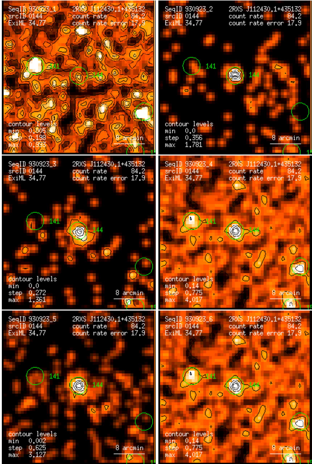
Figure 144: RASS 930923: detection 0144: band rate images, Gaussian filter: (1) PSPC channels 11 – 41, (2) 52 – 90, (3) 91 – 201, (4) 11 – 235, (5) 52 – 201, (6) 11 – 201. Broad band rates in counts/ks. Band rate contour levels in counts/ks/arcmin 2 .
