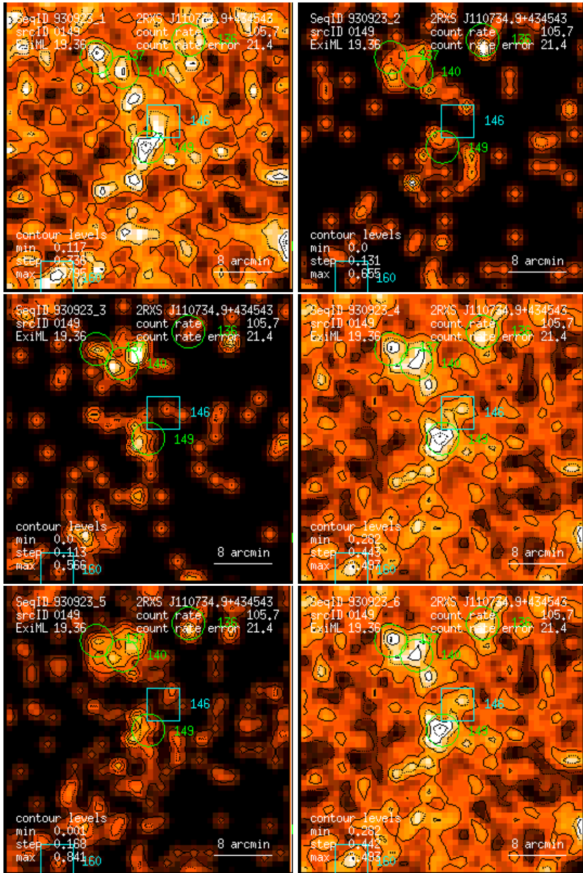
Figure 149: RASS 930923: detection 0149: band rate images, Gaussian filter: (1) PSPC channels 11 – 41, (2) 52 – 90, (3) 91 – 201, (4) 11 – 235, (5) 52 – 201, (6) 11 – 201. Broad band rates in counts/ks. Band rate contour levels in counts/ks/arcmin 2 .
