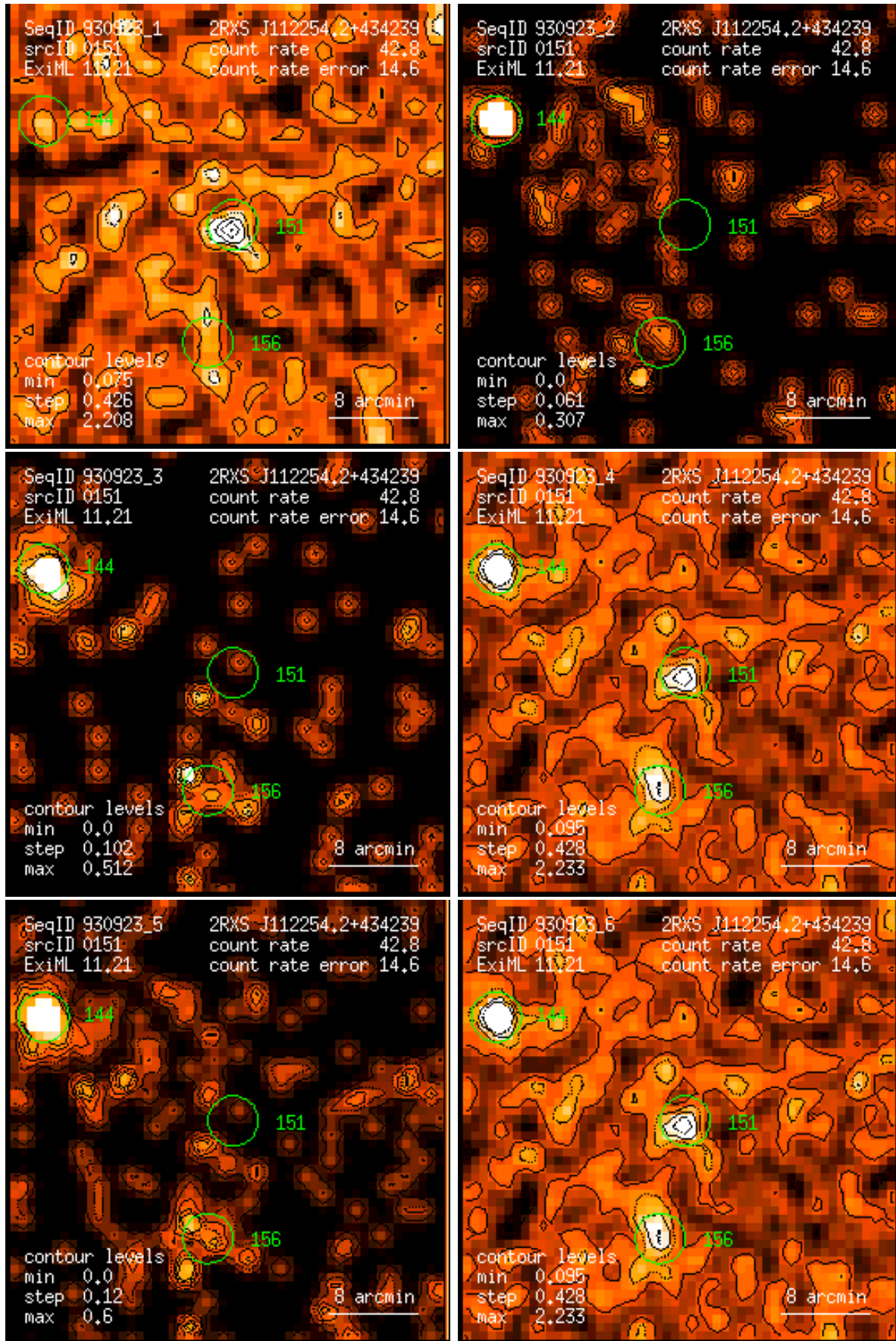
Figure 151: RASS 930923: detection 0151: band rate images, Gaussian filter: (1) PSPC channels 11 – 41, (2) 52 – 90, (3) 91 – 201, (4) 11 – 235, (5) 52 – 201, (6) 11 – 201. Broad band rates in counts/ks. Band rate contour levels in counts/ks/arcmin 2 .
