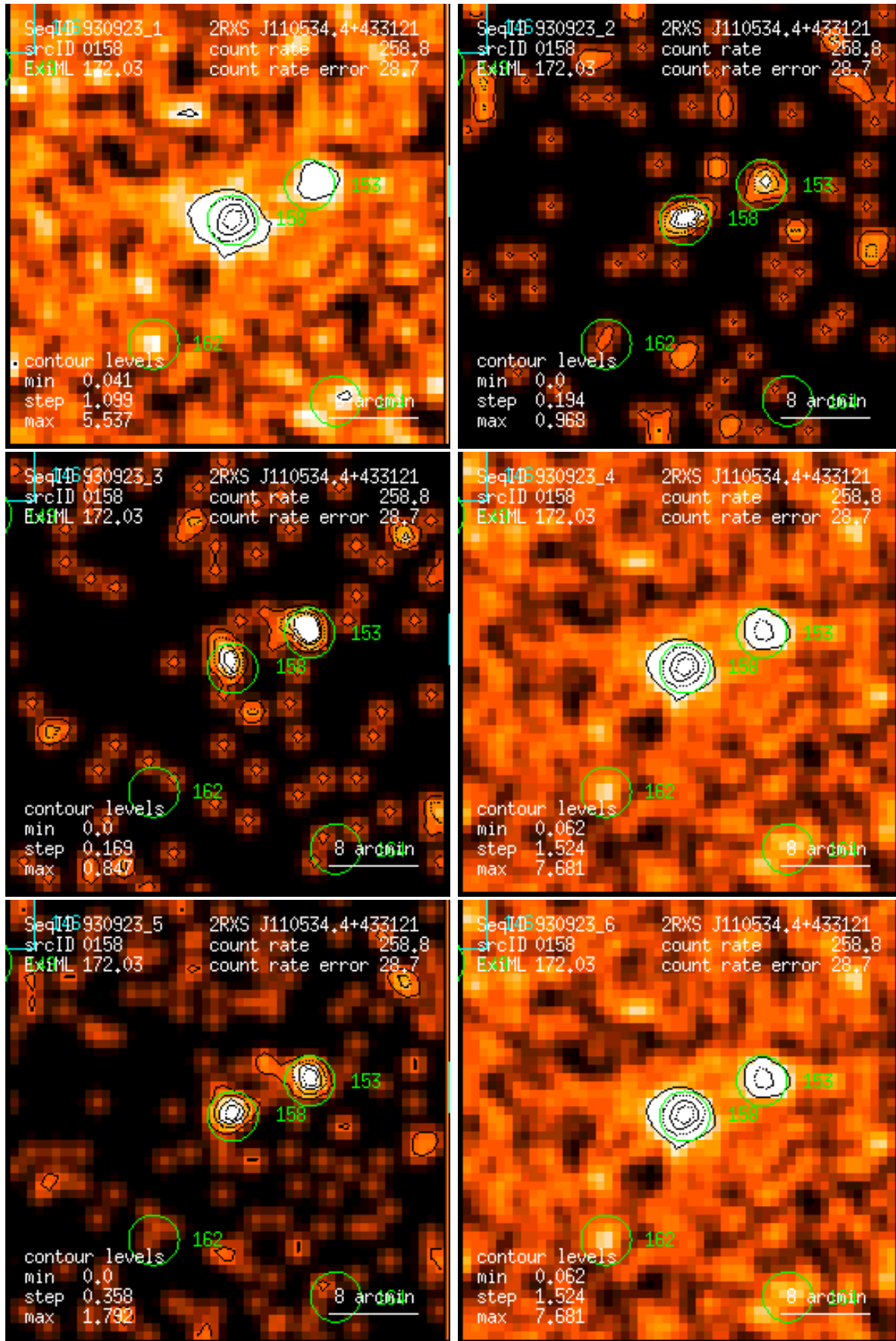
Figure 158: RASS 930923: detection 0158: band rate images, Gaussian filter: (1) PSPC channels 11 – 41, (2) 52 – 90, (3) 91 – 201, (4) 11 – 235, (5) 52 – 201, (6) 11 – 201. Broad band rates in counts/ks. Band rate contour levels in counts/ks/arcmin 2 .
