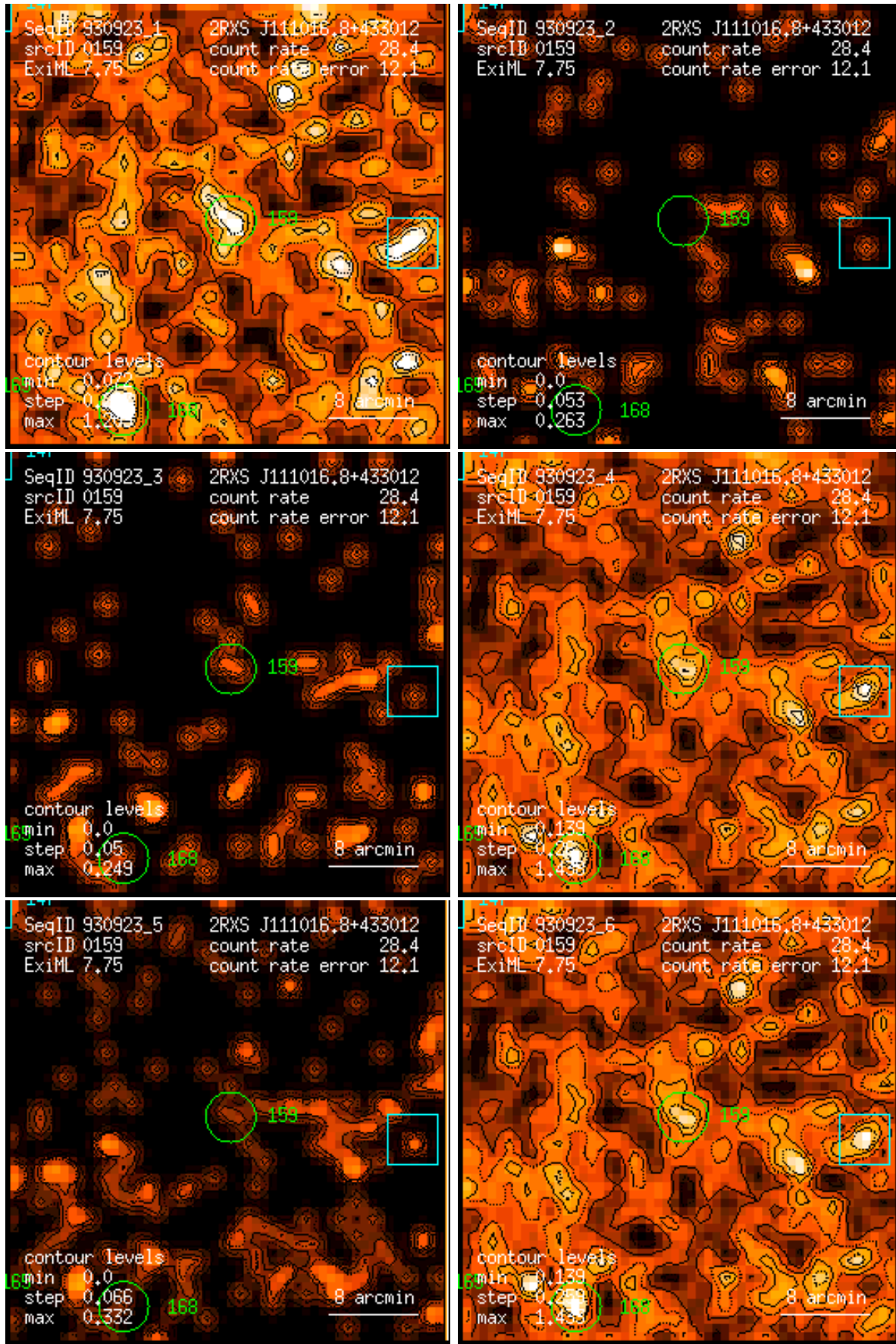
Figure 159: RASS 930923: detection 0159: band rate images, Gaussian filter: (1) PSPC channels 11 – 41, (2) 52 – 90, (3) 91 – 201, (4) 11 – 235, (5) 52 – 201, (6) 11 – 201. Broad band rates in counts/ks. Band rate contour levels in counts/ks/arcmin 2 .
