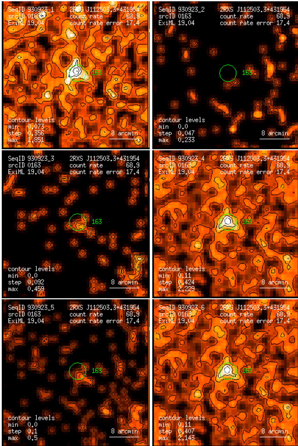
Figure 163: RASS 930923: detection 0163: band rate images, Gaussian filter: (1) PSPC channels 11 – 41, (2) 52 – 90, (3) 91 – 201, (4) 11 – 235, (5) 52 – 201, (6) 11 – 201. Broad band rates in counts/ks. Band rate contour levels in counts/ks/arcmin 2 .
